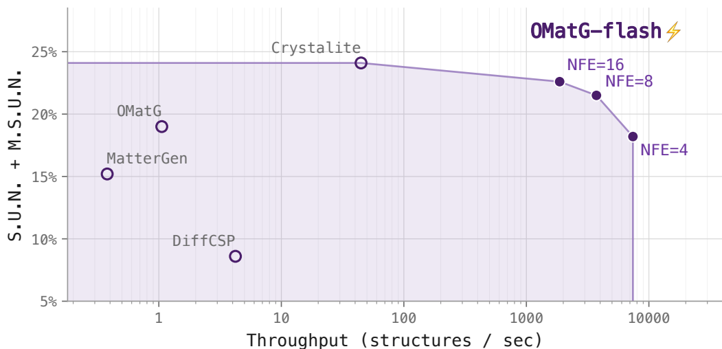
Figure 1: Pareto-Optimal Inference. Pareto frontier of combined S.U.N. and M.S.U.N. vs. throughput is shown for existing models. OMatG-flash is Pareto-optimal, surpassing existing models by an order of magnitude in terms of throughput while maintaining competitive raw performance on the DNG task. Solid points indicate OMatG-flash under several number of function evaluation (NFE) budgets.
