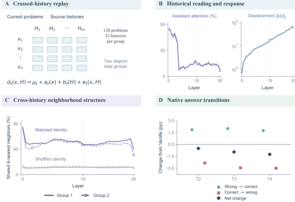
Figure 2: Historical computation after task switches in Qwen3-4B Instruct on MATH-500. A: Crossed-history replay with a frozen backbone. Each of two disjoint data groups crosses 128 current problems with 32 three-turn source histories. State displacement is decomposed into additive effects and an interaction response. B: Attention mass on earlier assistant-response bodies (left) and the norm of the current problem’s state displacement (right; logarithmic scale). C: Cross-history overlap of eight nearest candidate problems in interaction-response space, with the Question-identity shuffle control. At layer 19, interaction energy fractions are 0.69% and 0.66% for groups 1 and 2. In B and C, solid lines denote group 1; dashed lines with hollow squares denote group 2. Vertical dotted lines mark layer 19, reported in the text. Layers are zero-indexed. D: Native answer transitions relative to Vanilla T1, normalized by 2,000 pairs per turn. Wrong-to-correct contributions are positive and correct-to-wrong contributions negative. Diamonds mark net changes.
