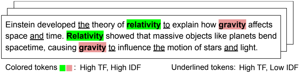
Figure 1: Illustration of TF-IDF weights applied to a short paragraph. Informative tokens such as relativity , and gravity receive higher weights, while common words like the and and are de-emphasized.
