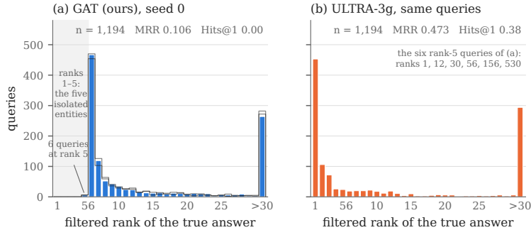
Figure 3: FBNEll, distribution of the filtered rank of the true answer over the 1,194 queries. (a) GAT seed 0 (bars) with seeds 1 and 2 as outlines; (b) ULTRA-3g on the same queries, same filter. Panel (a): no query lands at ranks 1–4: the five isolated entities occupy them; the six queries at rank 5 are the five whose answer is isolated and the one whose source is; the mode is rank 6. Panel (b): ULTRA-3g (MRR 0.473, Hits@1 0.38) has its mode at rank 1 and no gap; the six rank-5 queries of panel (a) land at ranks 1, 12, 30, 56, 156 and 530.
