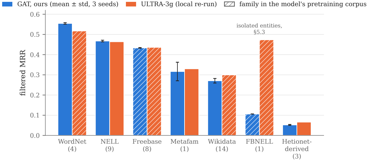
Figure 2: per-family filtered MRR, GAT (mean \pm std over 3 seeds) versus the re-run ULTRA-3g, families ordered from our strongest to weakest. Hatching marks a family present in the model’s own pretraining corpus; FBNELL is the isolated-entity split of Section 5.3.
