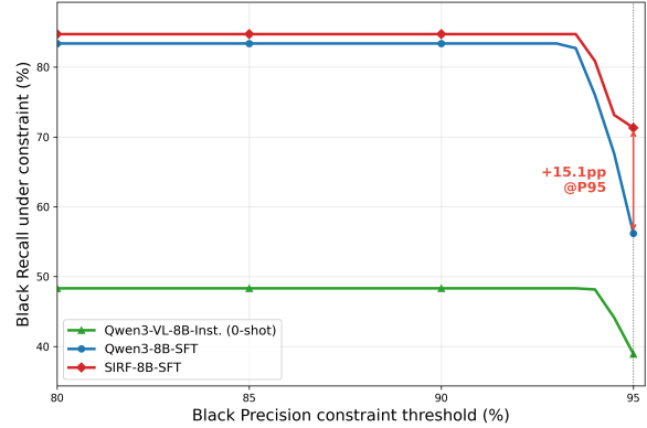
Figure 3: Black recall vs. precision constraint for the three same-source 8B arms (Qwen3-VL-8B-Inst. \rightarrow Qwen3-8B-SFT \rightarrow SIRF-8B-SFT); the gap is largest at P95 (+15.1pp).
