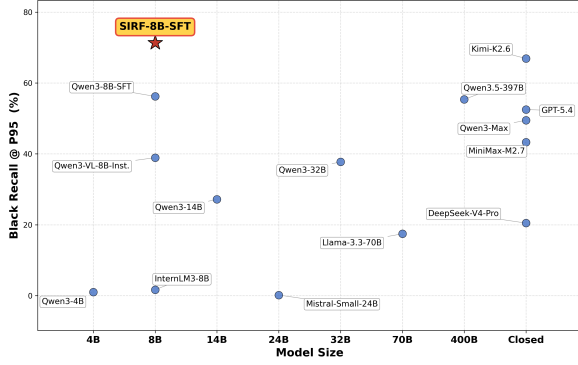
Figure 1: Black (risky) Recall@P95 vs. model size, among included, logprob-available models under this deployment interface. SIRF-8B sits above all compared open-weight (4B–400B) and closed-source models at the high-precision operating point. Excluded models: Claude, Doubao and GLM, whose APIs return no token logprobs, so no confidence ranking and hence no Recall@P can be computed; this is an interface limitation, not a capability judgment. Our core attribution to spec internalization does not rely on these cross-model comparisons but on the controlled 8B same-source study in Table 1.
