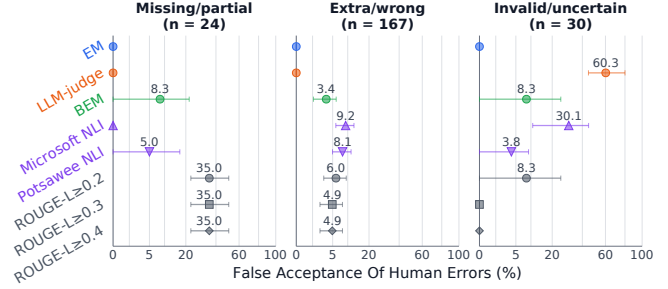
Fig. 3. Observed false-acceptance rates by human-annotated error category. All groups containing at least one error of the relevant category are included, covering 24/167/30 errors for missing/partial, extra/wrong and invalid/uncertain responses, respectively. Rates are averaged equally across included groups. Error bars show 95% confidence intervals derived from bootstrap sampling for 10,000 times.
