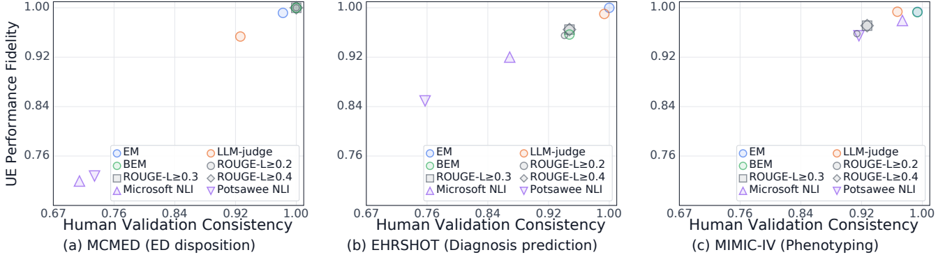
Fig. 2. Task-specific joint assessment of correctness criteria against the consensus audit. H is balanced accuracy averaged equally across three models; F is one minus absolute human-referenced AUROC distortion averaged across three models and four UE methods. Points use equal case weights within each group. Higher values indicate greater human agreement and UE performance fidelity, respectively.
