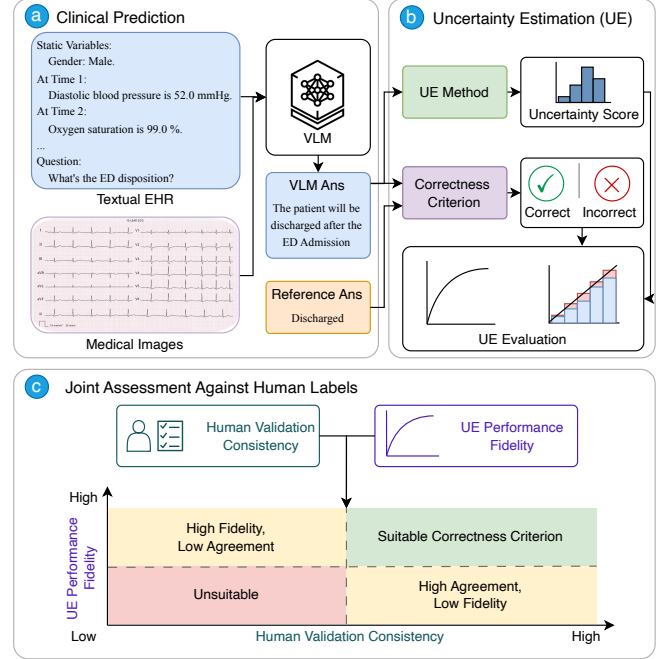
Fig. 1. Overview of the proposed evaluation framework. (a) A clinical model predicts from an EHR and, where available, an image. (b) An answer-only UE method assigns an uncertainty score, while a correctness criterion compares the prediction with the reference answer to define the binary outcome used for UE evaluation. (c) Joint assessment of agreement with human judgements and preservation of human-referenced UE performance.
