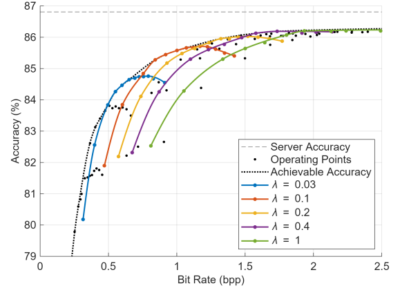
Fig. 8. Achieved rate-accuracy points of the proposed framework. Achievable accuracy is formed by connecting the Pareto-optimal operating points. Each solid line connects the operating points obtained with the same LIC model parameters while varying only \delta .
