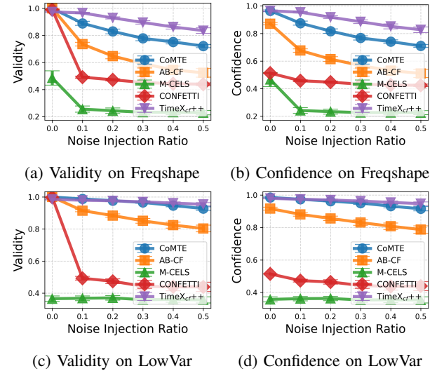
Fig. 4: The counterfactual explanations robustness analysis on Freqshape and LowVar.
