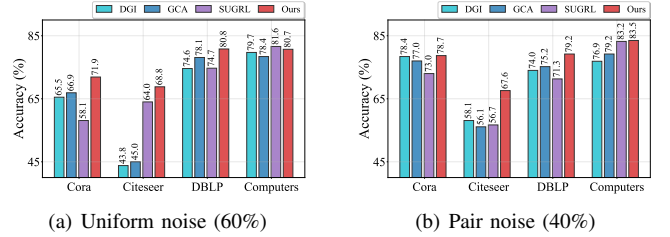
Fig. 3: Node classification performance of PASTA with different annotators under the highest noise rates for uniform and pair noise.
