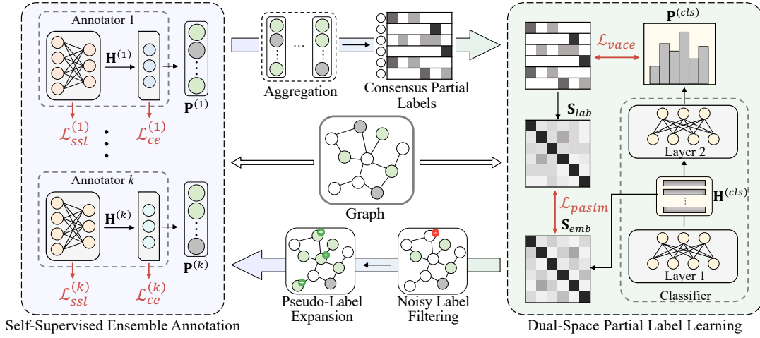
Fig. 2: The framework of the proposed PASTA. On the left, we leverage diverse self-supervised graph learning algorithms to construct annotators and generate consensus labels. On the right, we introduce \mathcal{L}_{pasim} and \mathcal{L}_{vace} to guide the classifier in learning robust patterns from the consensus labels. The trained classifier is then used to filter and expand dataset labels, which are subsequently used to further optimize the annotators' predictors. Finally, the two modules are iteratively optimized.
