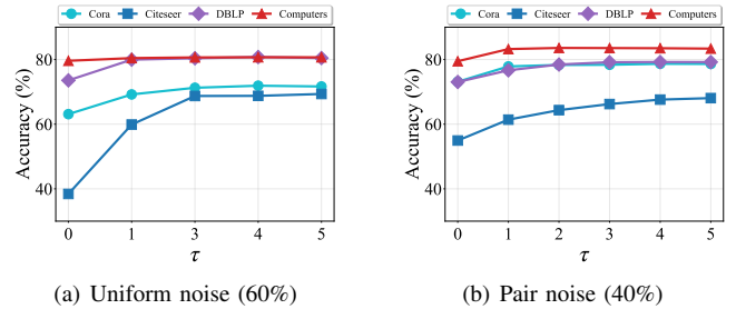
Fig. 4: Sensitivity Analysis of the Parameter \tau in PASTA.
