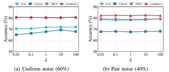
Fig. 6: Sensitivity Analysis of the Parameter \lambda in PASTA.
