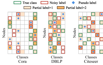
Fig. 5: Visualization of consensus partial label and one-hot pseudo-label (ten sampled noisy nodes).
