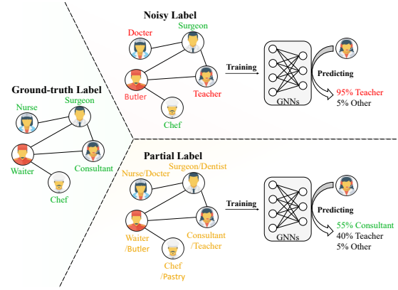
Fig. 1: Sketch maps of noisy label and partial label learning. While noisy labels tend to drive the model toward confident but potentially incorrect predictions, partial labels help the model produce ambiguous yet more accurate predictions.
