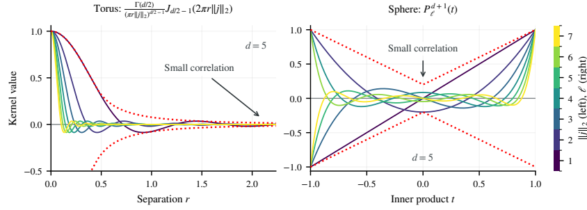
Figure 2: Left: the normalized Bessel factor as a function of the pairwise separation r . Right: the normalized Gegenbauer polynomial P_\ell^{d+1}(t) as a function of the inner product t , both for d = 5 . Colors identify the frequency norm \|j\|_2 (left) or the degree \ell (right), from 1 to 7; the constant mode is omitted. Dotted red curves show the envelope of each family, and arrows mark the regions of low correlation that motivate the surrogate.
