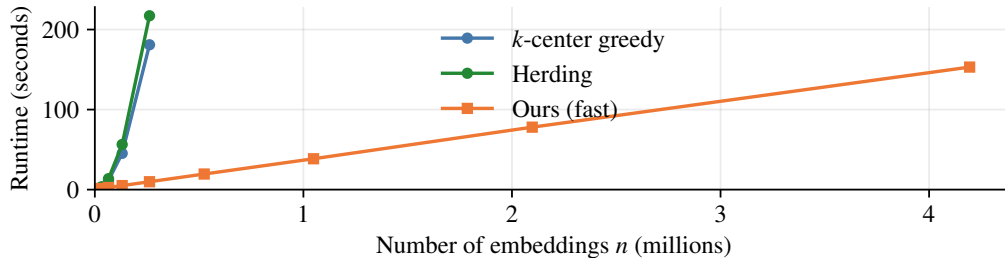
Figure 4: Recorded runtime versus input size (linear axes). We select n/128 points from standard-normal, 4096-dimensional float32 embeddings on an NVIDIA GeForce RTX 5090. We use binary representations with 64k bits.
