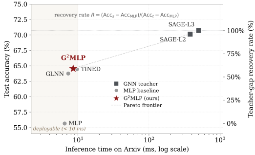
Figure 3: Inference time on Arxiv ( \sim 170K nodes).
