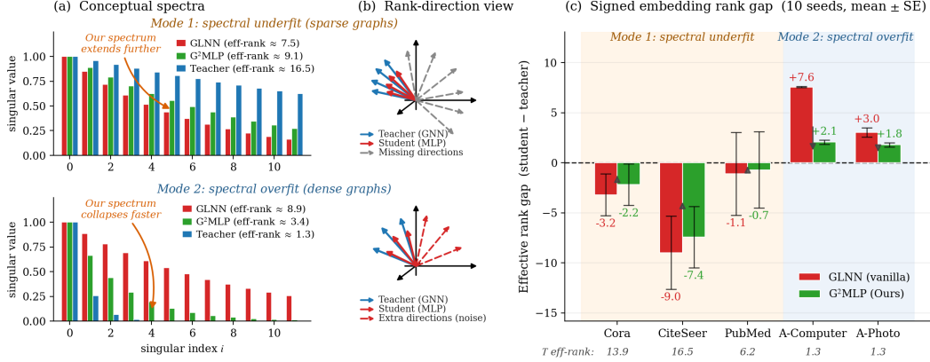
Figure 1: Two spectral failure modes of GNN-to-MLP distillation. (a) Singular-value spectra: GLNN exhibits spectral underfit on sparse graphs and spectral overfit on dense graphs. (b) Rank-direction sketch. (c) Per-dataset rank gap.
