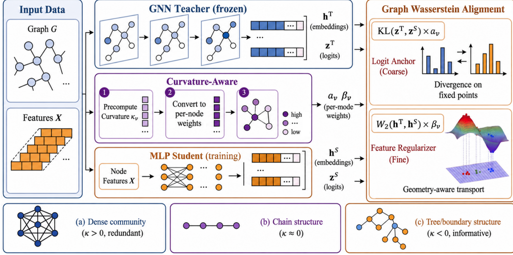
Figure 2: Overview of G^2 MLP. A frozen GNN teacher and an MLP student produce embeddings and logits; precomputed Ollivier–Ricci curvature yields per-node weights \alpha_v and \beta_v that allocate prediction-level and representation-level alignment during training.
