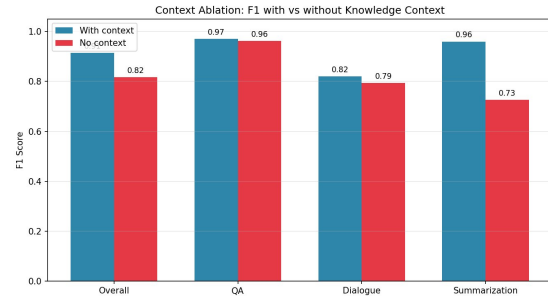
Figure 2: F1 with and without knowledge context across tasks. Summarization depends most on context ( -24\% ); QA is largely self-contained ( -1\% ).
