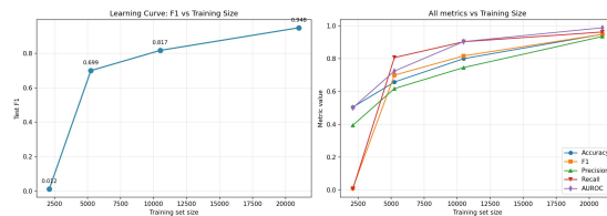
Figure 3: Learning curves: F1 (left) and all metrics (right) versus training set size. A sharp elbow at \sim 5K examples captures most of the discriminative signal.
