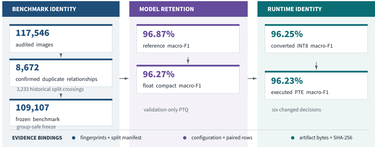
Figure 1: CropCop audit-to-runtime evidence chain.
