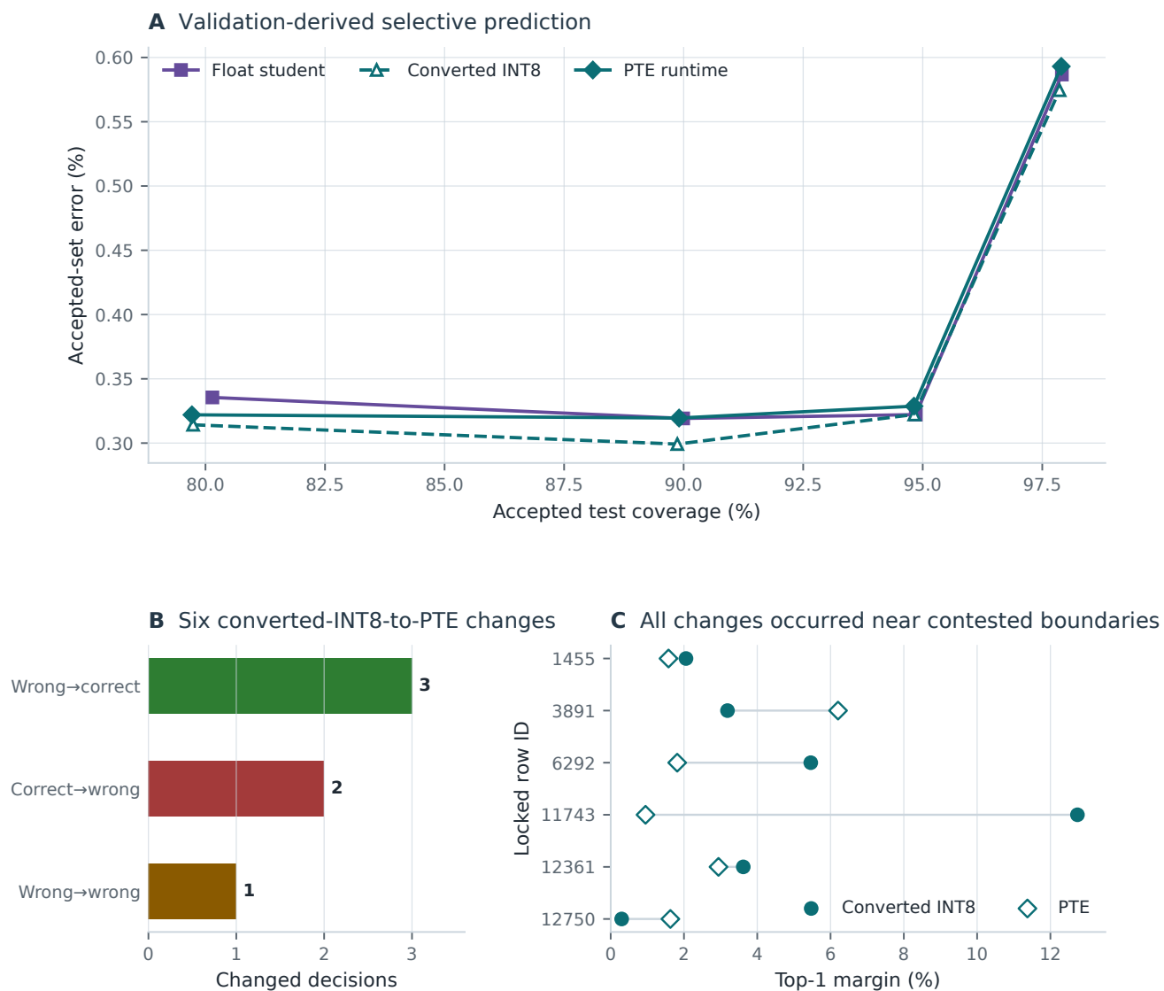
Figure 6: Validation-derived selective-prediction operating points and the six converted-INT8-to-PTE decision changes.
