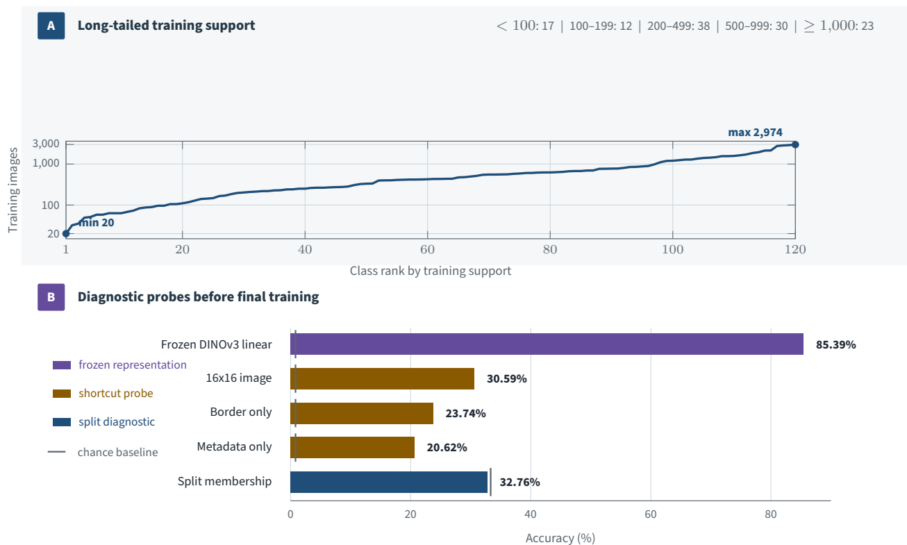
Figure 3: Long-tail training support and pre-training diagnostic probes.
