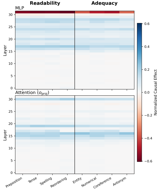
Figure 4: Last Token mode causal tracing on Prometheus across all eight attacks. Top row: MLP causal effects; bottom row: Attention o_{proj} causal effects.
