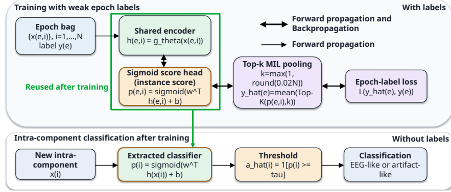
Fig. 2: Weakly supervised MIL-based intra-component classifier. During training, each EEG epoch is treated as a bag of intra-components. A shared encoder maps each intra-component to an embedding, and a sigmoid head assigns an instance-level artifact-likeness score. The highest-scoring 2% of intra-components are averaged by top- k MIL pooling to obtain the epoch-level contamination score, which is optimized against the weak epoch label. After training, the MIL pooling layer is discarded, and the encoder and score head are reused for intra-component classification. The framework permits threshold selection on validation data, while the proof-of-concept cleaning evaluation used a fixed threshold of \tau = 0.5 to define a binary attenuation mask.
