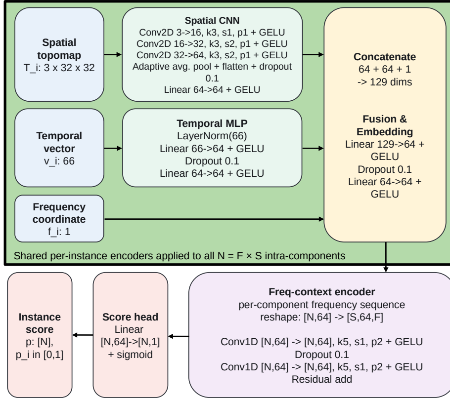
Fig. B.1: Detailed architecture of the intra-component classifier. Each intra-component has three inputs: a 3-channel spatial topomap T_i \in \mathbb{R}^{3 \times 32 \times 32} , a 66-dimensional hand-crafted temporal feature vector v_i \in \mathbb{R}^{66} , and a normalized scalar frequency coordinate f_i \in \mathbb{R} . Kernel size, stride, and padding are denoted by k , s , and p , respectively. The spatial CNN, temporal MLP, and fusion modules are shared per-instance encoders applied to all N = F \times S intra-components, where F is the number of frequency bins and S is the number of ILRMA sources, as indicated by the green block. The frequency-context encoder then gathers all embeddings in the bag (one EEG epoch), reshapes them to [S, 64, F] , and applies 1-D convolutions along the frequency axis for each component (ILRMA source). Each final score p_i is therefore an intra-component artifact-likelihood score; one EEG epoch produces N such scores.
