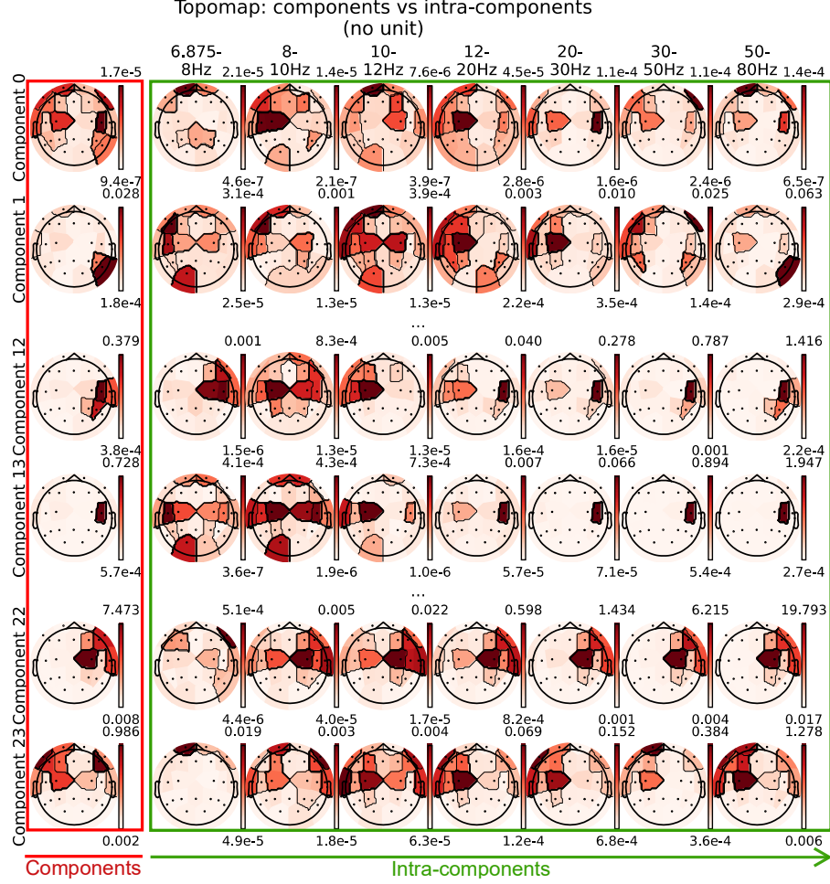
Fig. 1: Unfolding components to intra-components with components 0, 1, 12, 13, 22 and 23 as examples. For visual clarity, frequency bins are aggregated into standard EEG frequency bands: theta (6.875–8 Hz; corresponding to the available portion of the conventional 4–8 Hz theta band), low-alpha (8–10 Hz), high-alpha (10–12 Hz), low-beta (12–20 Hz), high-beta (20–30 Hz), low-gamma1 (30–50 Hz), and low-gamma2 (50–80 Hz). Following [19], the ILRMA decomposition starts at 6.875 Hz to avoid linear dependencies across frequency; each topomap uses an individual color scale to show its spatial distribution; the numbers beside each topomap are the limits of its color range for unitless, rescaled projected power; hence, colors are not quantitatively comparable across maps. The intra-component representation enables frequency-wise separation of mixed neural and non-neural activity within components.
