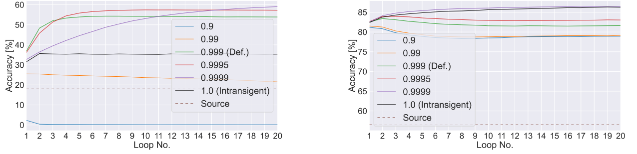
Figure A.7: Mean accuracy [%] for each loop of common testing sequence on ImageNet-C (L) using CoTTA ( left ) and on CIFAR10-C (L) using AdaContrast ( right ). The brown dashed line indicates the source model accuracy.
