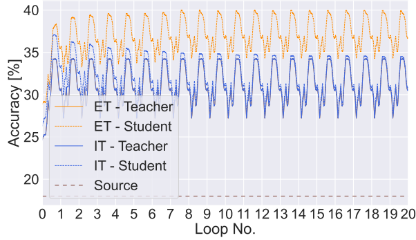
(e) PETAL, ResNet50
