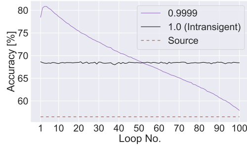
Figure A.4: Mean accuracy [%] of CoTTA with varying \beta for each loop of common CIFAR10-C testing sequence repeated 100 times. The brown dashed line indicates the accuracy of the source model as a reference.
