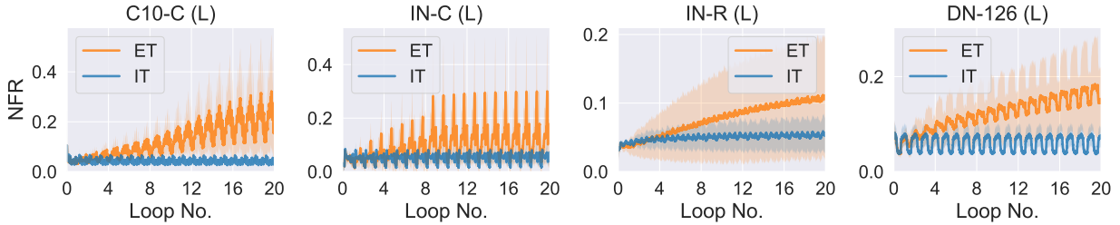
Figure 8: Per-batch Negative Flips Rate (NFR) of the student model averaged over AdaContrast, CoTTA, RoTTA and PETAL methods (ET) on each dataset, along with their IT-enhanced versions (IT). The shaded regions represents \pm standard deviation illustrating the variability across methods.
