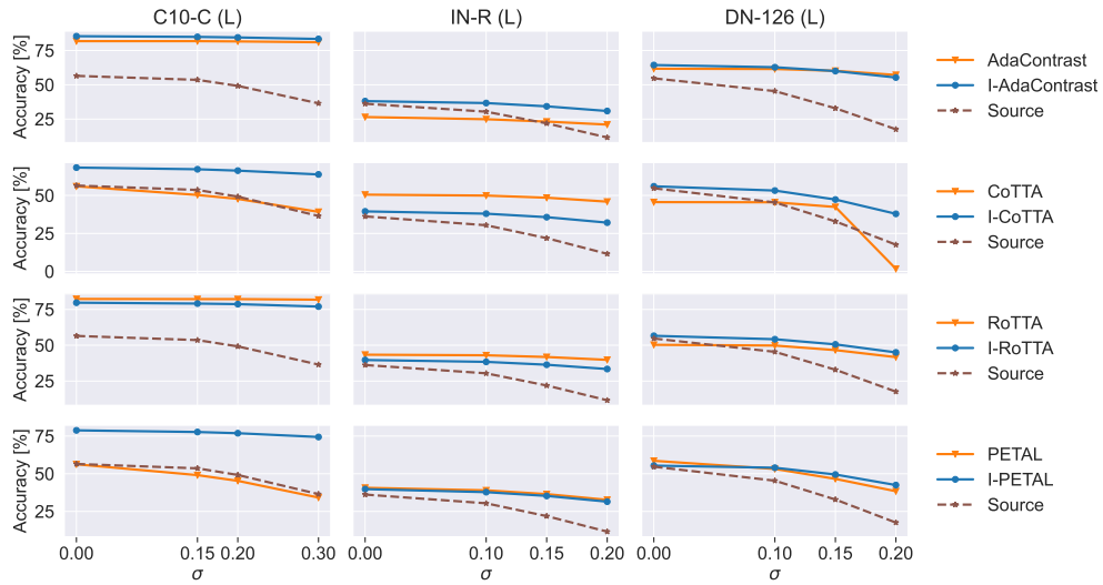
Figure A.3: The overall average accuracy on each of the tested benchmarks of the original methods and IT-enhanced versions using source model weights perturbed using Gaussian noise with increasing standard deviation \sigma . The \sigma = 0 indicates the performance of the model not perturbed by noise. The brown dashed line indicated the source model accuracy.
