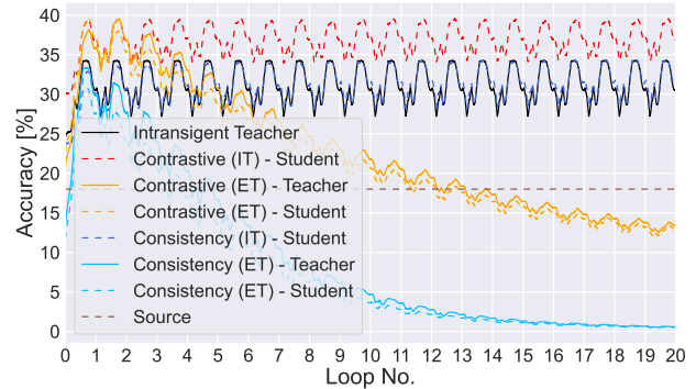
Figure 2: Per-batch accuracy on repeated ImageNet-C (20 loops) with EMA teacher (ET) and intransigent teacher (IT), both for teacher (solid) and student (dashed). Only the self-supervised losses, without any additional components (or restart mechanisms), allow for successful adaptation over long sequences when the teacher is intransigent.
