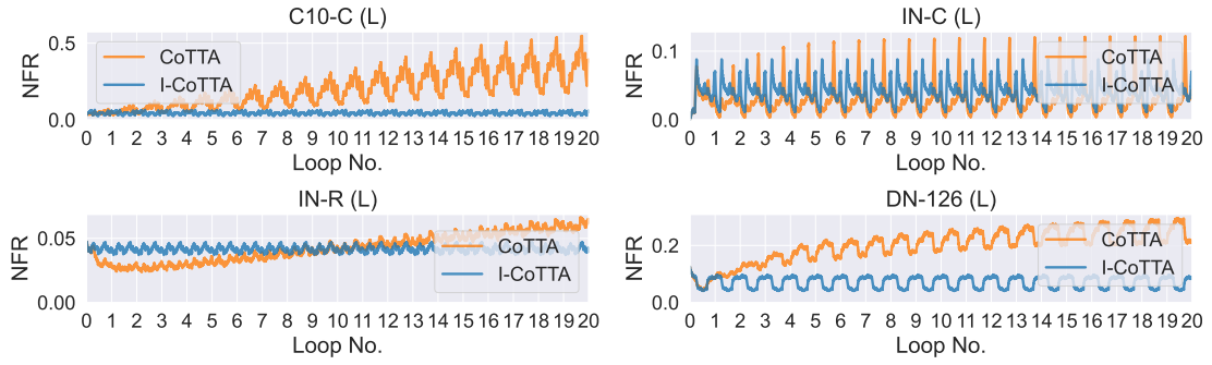
(b) CoTTA
