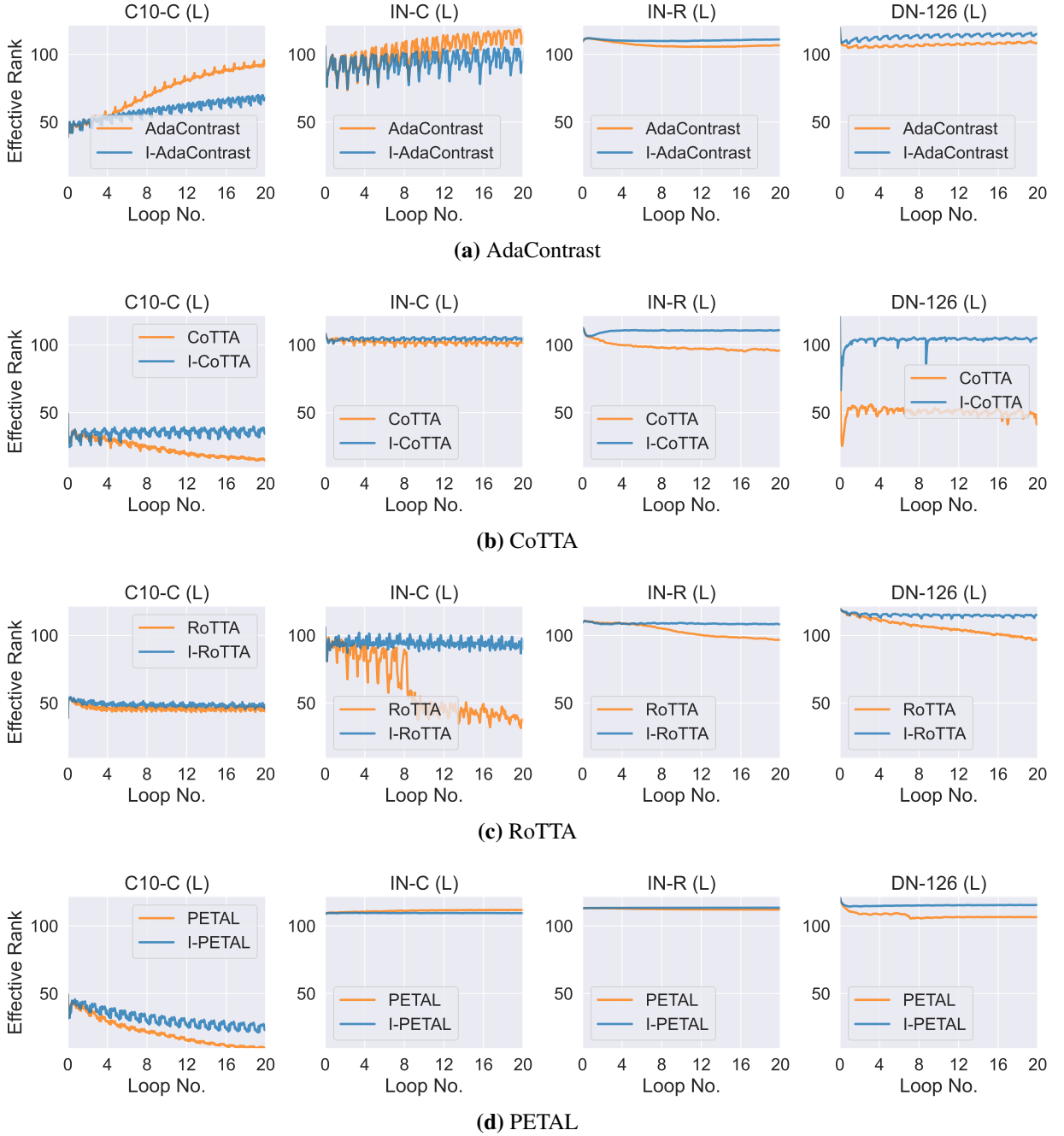
Figure A.1: Effective rank values of the features extracted from the student model during the TTA every 50 batches on each benchmark using AdaContrast (a), CoTTA (b), RoTTA (c) and PETAL (d) methods and IT-enhanced version.
