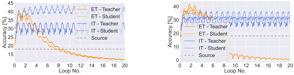
Figure 7: Per-batch accuracy on repeated ImageNet-C (20 loops) using ResNet50. AdaContrast ( left ) and RoTTA ( right ) are compared with an EMA teacher (ET, orange) and our intransigent teacher (IT, blue), both for teacher (solid) and student (dashed). The EMA teacher visibly suffers from error accumulation as the sequence gets longer. After the 3rd loop, IT manages to avoid model collapse and, surprisingly, the student performs significantly better.
