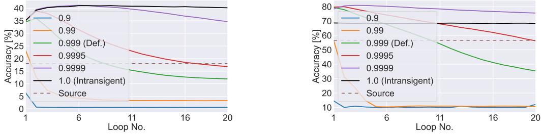
Figure 3: Mean accuracy [%] for each loop of common testing sequence on ImageNet-C (L) with AdaContrast ( left ) and CIFAR10-C (L) with CoTTA ( right ). The brown dashed line indicates the source model accuracy as a reference.
