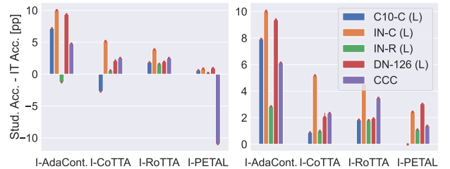
Figure 6: Accuracy difference between student and intrasentient teacher in percentage points, with default learning rate values (left) and after parameter search (right).
