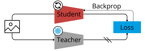
Figure 4: The Intransigent Teacher. The student’s weights are updated using gradient-based optimization, while the teacher’s weights remain fixed throughout adaptation.
