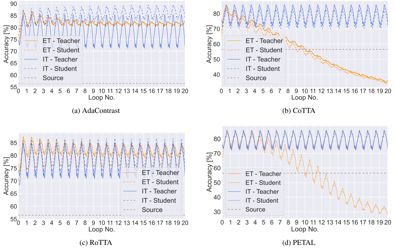
Figure A.10: Per-batch accuracy [%] on CIFAR10-C (L) using WideResNet-28. Comparison with EMA teacher (ET, orange) and intransigent teacher (IT, blue), for both teacher (solid) and student (dashed).
