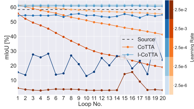
Figure A.2: Segmentation results (mIoU [%]) for each repeated day2night sequence on CarlaTTA (Marsden et al., 2024b). Orange and blue colors indicate CoTTA and I-CoTTA, respectively. The darker the color, the higher the learning rate value used to achieve the result. The black dashed line indicates the source model performance as a reference.
