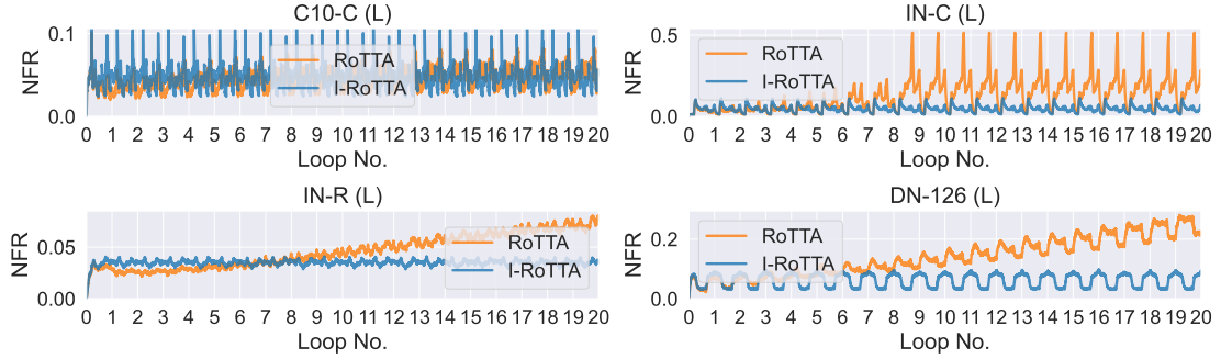
(c) RoTTA
