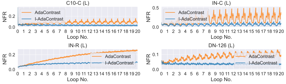
(a) AdaContrast
