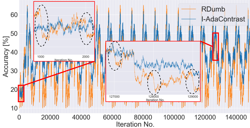
Figure A.5: Batch-wise accuracy plots of RDumb and I-AdaContrast methods on ImageNet-C (L) benchmark. The accuracy values were smoothed to make the plot clearer. RDumb resets the model every 1000 iterations, which causes significant drops in accuracy after the reset.
