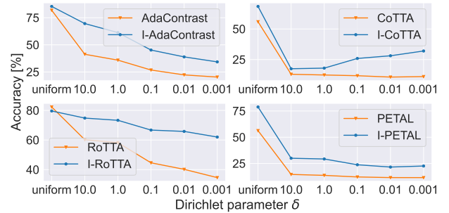
Figure 5: Classification accuracy on CIFAR10-C (L). Samples are sorted by class for different levels of correlation, by varying the Dirichlet concentration parameter \delta .
