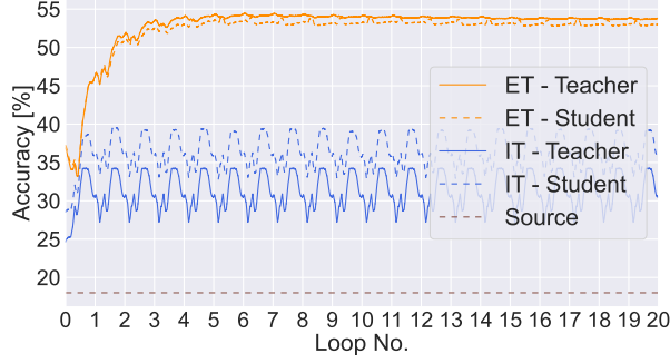
(a) CoTTA, ResNet50
