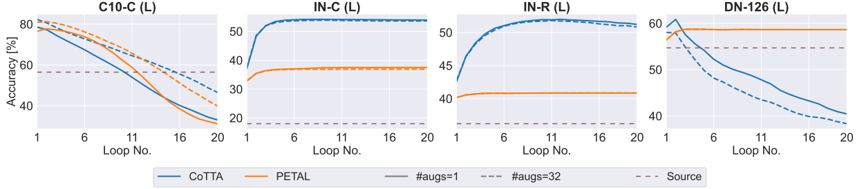
Figure A.6: Mean accuracy [%] for each loop of the common testing sequence on CIFAR10-C (L), ImageNet-C (L), ImageNet-R (L), and DomainNet-126 for CoTTA and PETAL. Methods are tested with pseudo-labels generated by averaging across predictions on either 1 or 32 randomly augmented images. The brown dashed line indicates the source model accuracy as a reference.
