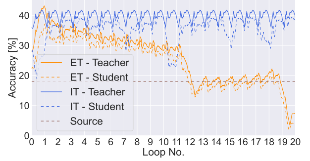
(b) CoTTA, ViT-B16
