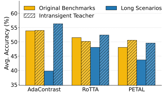
Figure 1: Average classification accuracy [%] for the baseline methods, with and without our Intransigent Teacher technique, evaluated across the original benchmarks and their long variants (20× repetitions). While baseline methods exhibit performance degradation as test sequence length increases, our Intransigent Teacher modification to the teacher-student framework effectively mitigates this decay and maintains robust accuracy.
