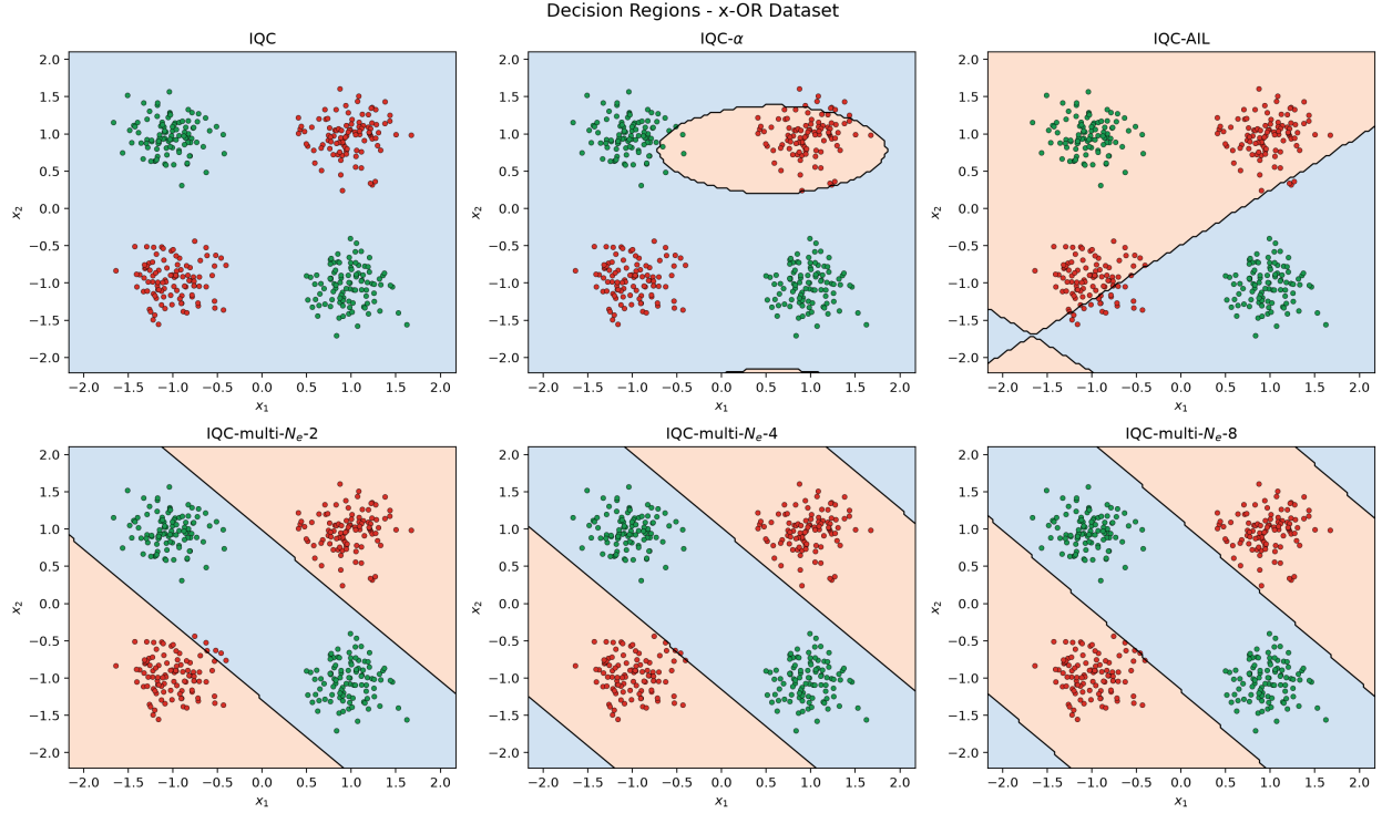
Figure 6: Decision regions learned by the six IQC variants on the XOR dataset. The multidimensional variants generate structured alternating regions that separate the four data clusters.
