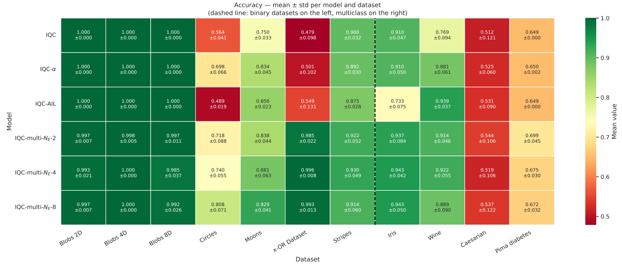
Figure 2: Accuracy (mean \pm standard deviation) obtained by each IQC variant across the eleven benchmark datasets. The dashed vertical line separates binary datasets (left) from multiclass datasets (right).
