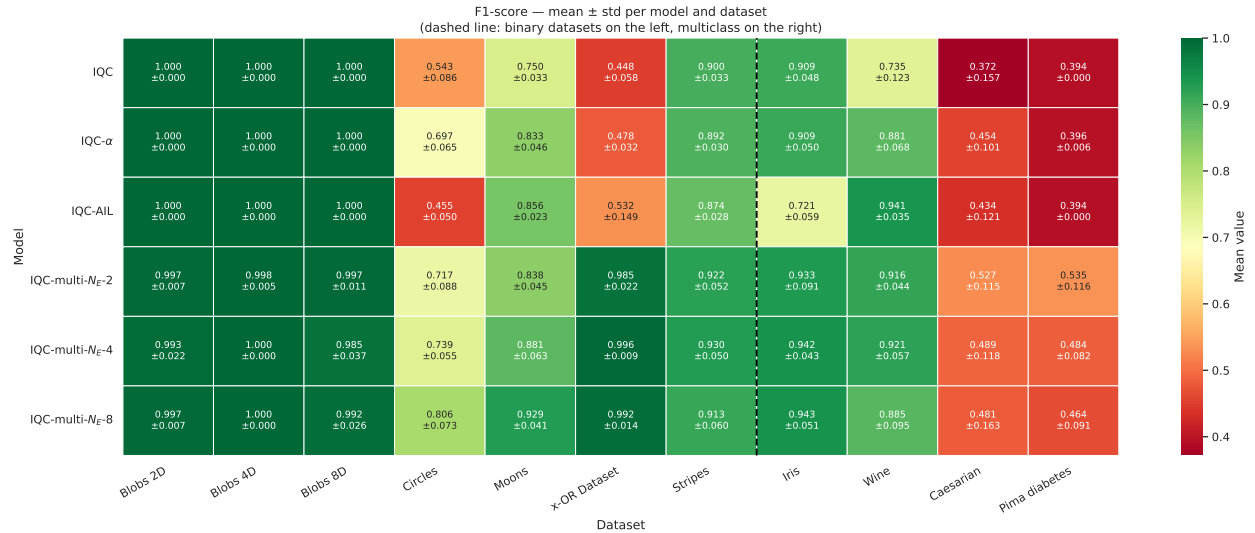
Figure 3: F1-score (mean \pm standard deviation) obtained by each IQC variant across the eleven benchmark datasets. The dashed vertical line separates binary datasets (left) from multiclass datasets (right).
