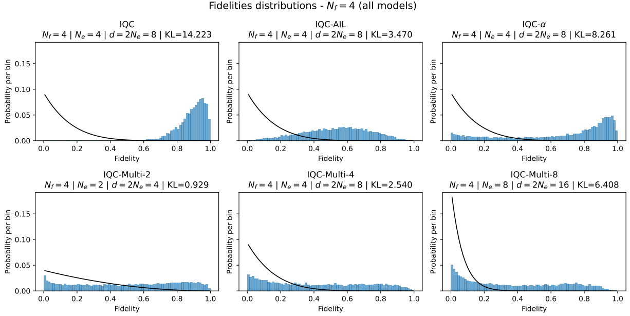
Figure 7: Empirical fidelity distributions for the six IQC models at N_f = 4 , together with the corresponding Haar reference distributions. The values of N_e , the global Hilbert-space dimension, and the KL divergence are indicated for each model.
