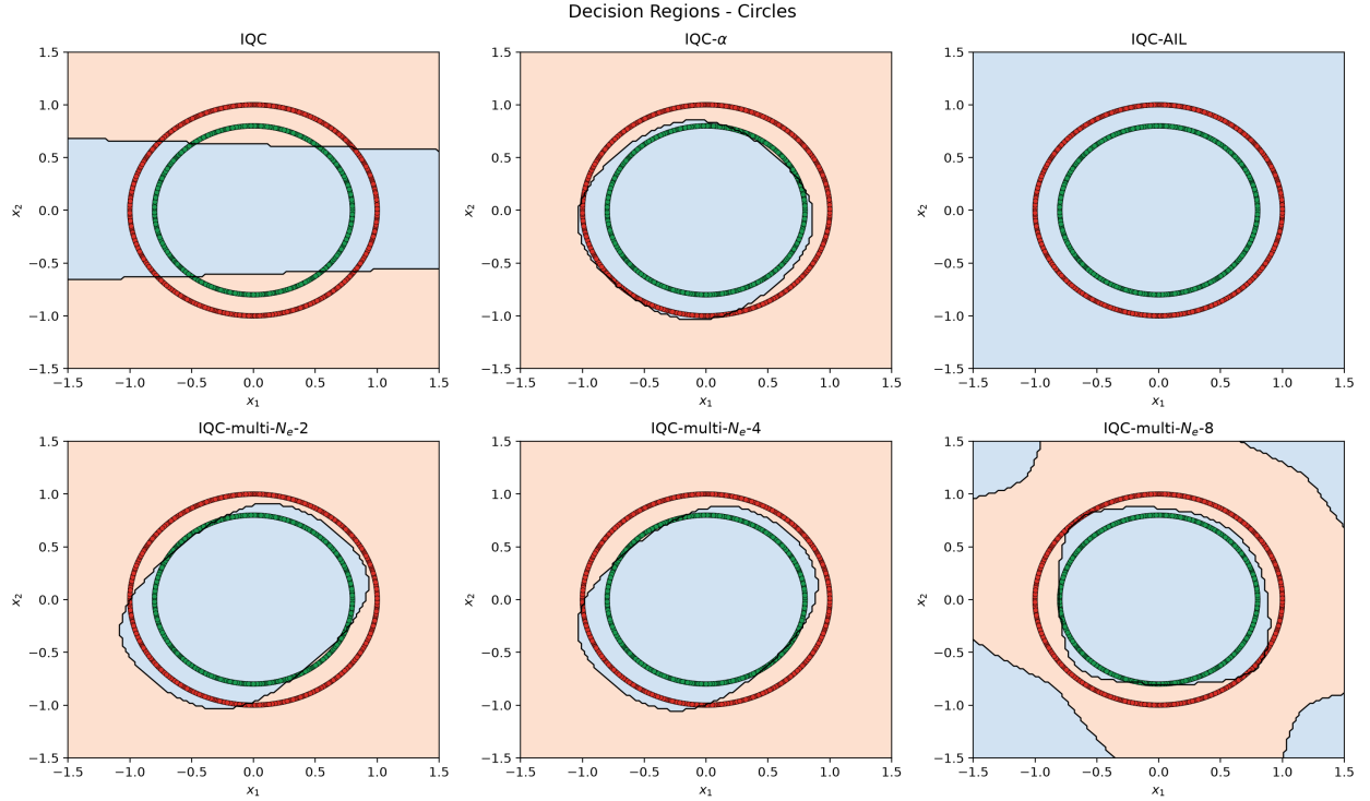
Figure 4: Decision regions learned by the six IQC variants on the Circles dataset. The plots show the resulting classification regions together with the data points for the two classes.
