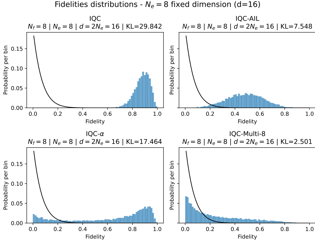
Figure 9: Fidelity distributions for the four models with N_f = 8 and the same global Hilbert-space dimension, d = 16 , together with the common Haar reference distribution.
