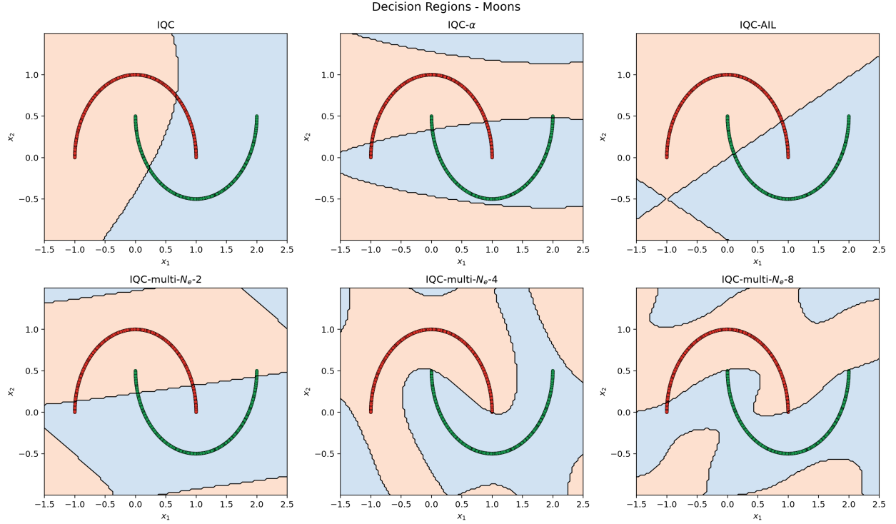
Figure 5: Decision regions learned by the six IQC variants on the Moons dataset. The plots show the resulting classification regions together with the data points for the two classes.
