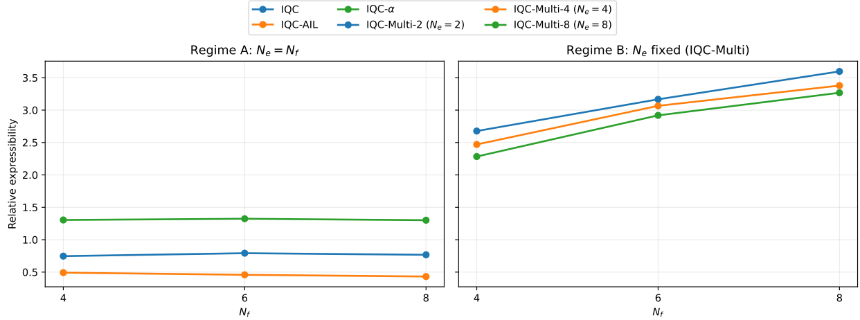
Figure 8: Relative expressibility as a function of the number of input features N_f . Left: IQC, IQC-AIL, and IQC- \alpha with N_e = N_f . Right: IQC-Multi models with fixed environment dimensions N_e = 2, 4 , and 8 .
