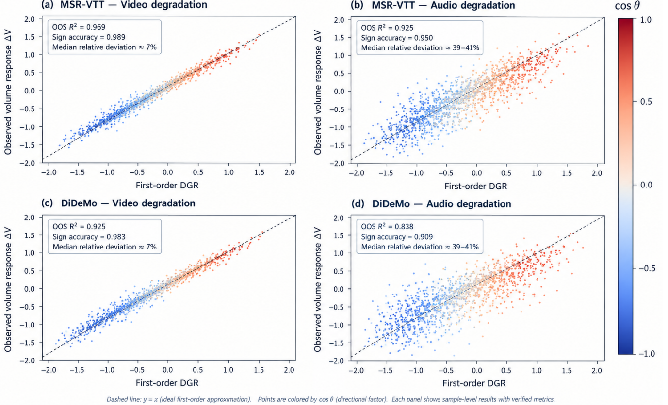
Fig. 5. Pointwise validation of the Directional Geometric Response. Each panel compares the observed volume response \Delta V with the first-order directional quantity \text{DGR} = \nabla V(\mathbf{o}_c)^\top \Delta \mathbf{o} for one dataset–degradation cell. The dashed diagonal denotes the ideal first-order correspondence \Delta V = \text{DGR} . The strong alignment across samples confirms that the directional first-order term captures the dominant response structure, while the visible deviations from the diagonal, particularly for the audio axes, quantify non-negligible higher-order effects.
