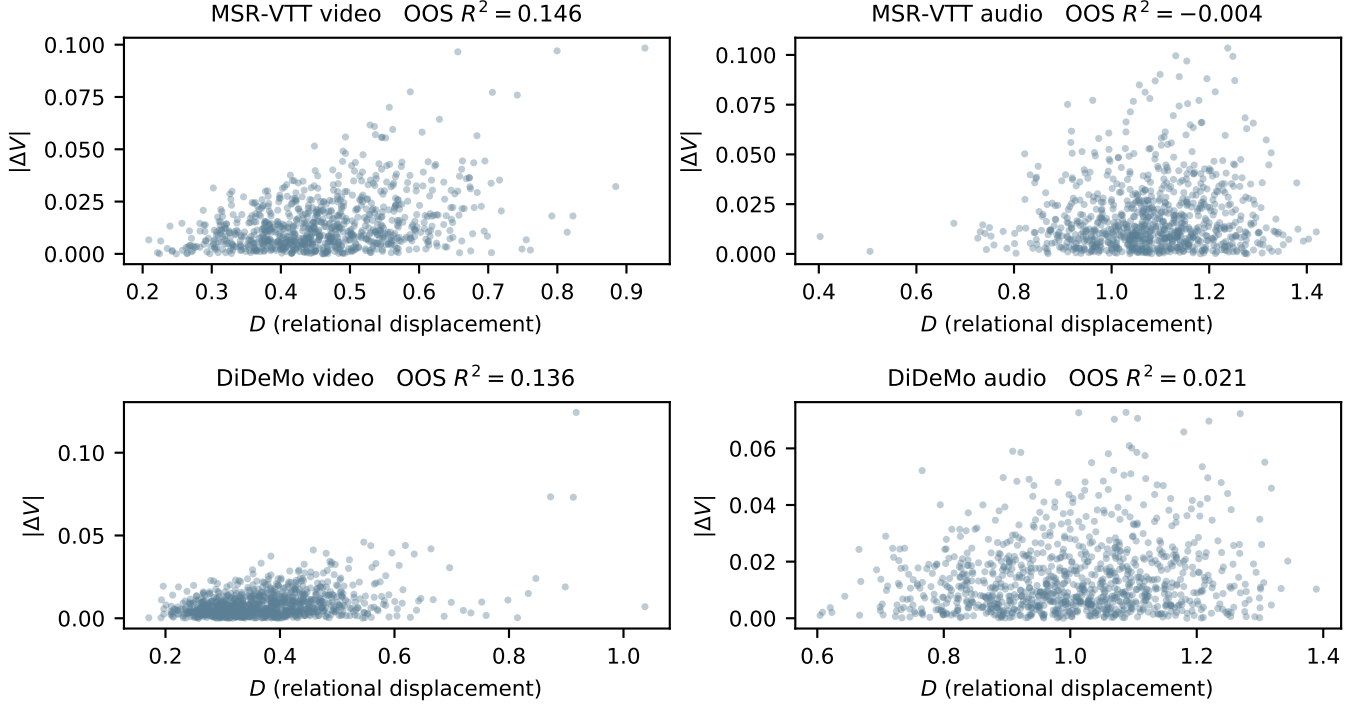
Fig. 3. Absolute volume response |\Delta V| versus relational displacement magnitude D under single-axis degradation (top: MSR-VTT; bottom: DiDeMo; left: video blur; right: audio noise). Magnitude leaves most of the response variance unexplained, and magnitude-matched samples respond systematically differently.
