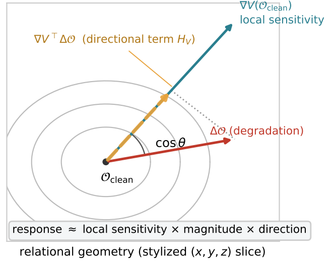
Fig. 2. Local geometric decomposition of the first-order response. A degradation moves the relational geometry by \Delta \mathbf{o} from the clean operating point \mathbf{o}_c ; the induced volume change is governed by the projection of \Delta \mathbf{o} onto the local gradient \nabla V(\mathbf{o}_c) , i.e., local gain g_V \times magnitude D \times \cos \theta .
