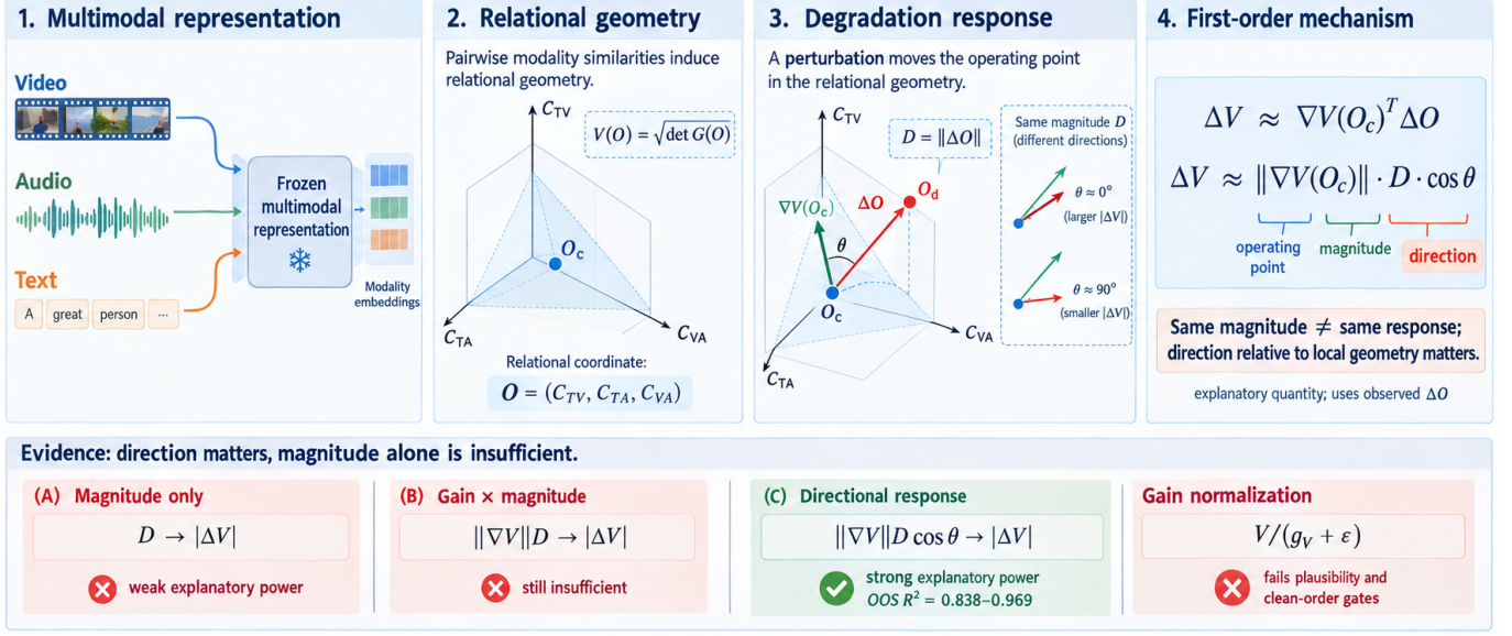
Fig. 1. Mechanism overview of direction-dependent responses in multimodal geometric representations. A clean multimodal representation defines an operating point O_c in relational geometry; a controlled degradation produces a displacement \Delta O , and the first-order volume response is governed jointly by the local operating-point gain \|\nabla V(O_c)\| , the displacement magnitude D = \|\Delta O\| , and the direction factor \cos \theta , whose product defines the Directional Geometric Response (DGR). Empirically, magnitude alone provides weak response predictability, the direction-free gain-magnitude product remains insufficient, and the direction-aware first-order quantity explains substantially more of the response heterogeneity. DGR is an explanatory quantity because it uses the observed degraded-state displacement.
