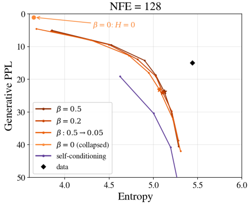
(c) Reinforce-DMD, NFE = 128
