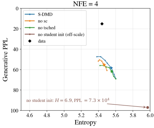
(a) Simplex-DMD, NFE = 4
