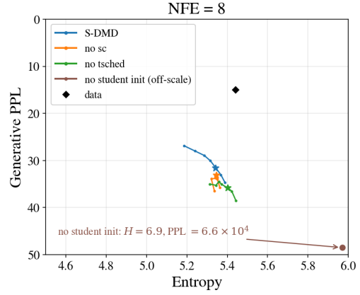
(b) Simplex-DMD, NFE = 8
