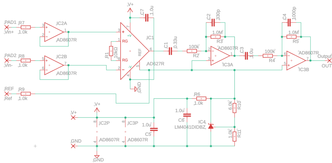
Supplementary Figure 1: Circuit diagram of the EMG amplification system. A voltage follower (AD8607, Analog Devices) was placed after the electrode, followed by a differential amplifier (AD627, Analog Devices) with a gain of 25. EMG signals were further amplified to 2,500 using subsequent operational amplifiers. Four identical circuits were integrated into the device.
