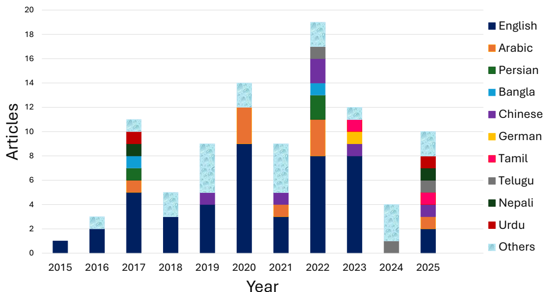
FIGURE 9: Trends in language-specific OCR models.
