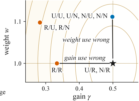
Figure 3: Each use has its own reference value. (a) Policies, written gain use/weight use; the marks rate each use’s gradient ( \approx : on average over the new rounding, the forward fixed; N/N hands both uses one new rounding). U/R is the reference; ★: matches it at both uses, at least on average. (b) Where each policy’s average update is zero in the two-parameter model of Section 3.2: ★ marks the minimum of the expected loss (shading); vermilion dots: the gain use reads R .
