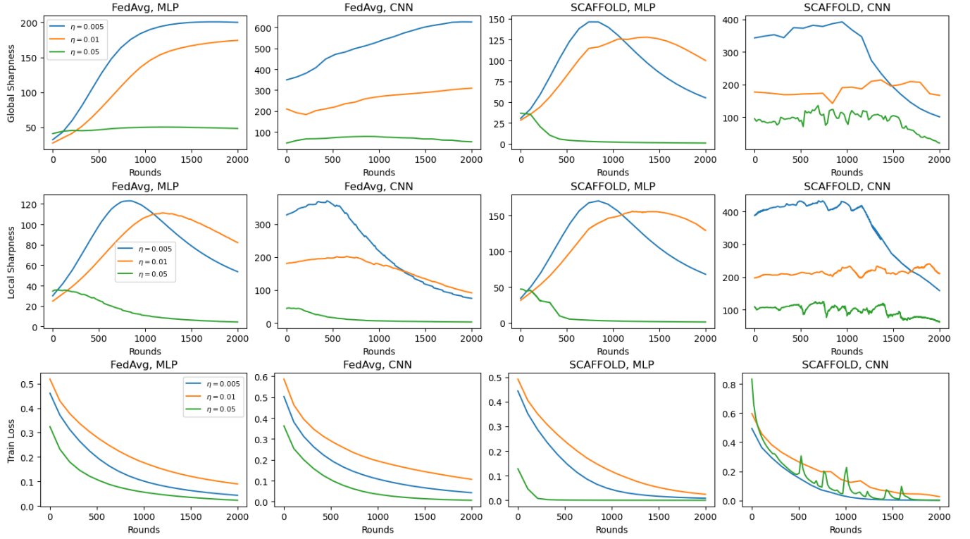
Figure 6: FashionMNIST global sharpness (top), local sharpness (middle), and train loss (bottom) over train trajectories with both SCAFFOLD and FedAvg and with both MLP and CNN architectures.
