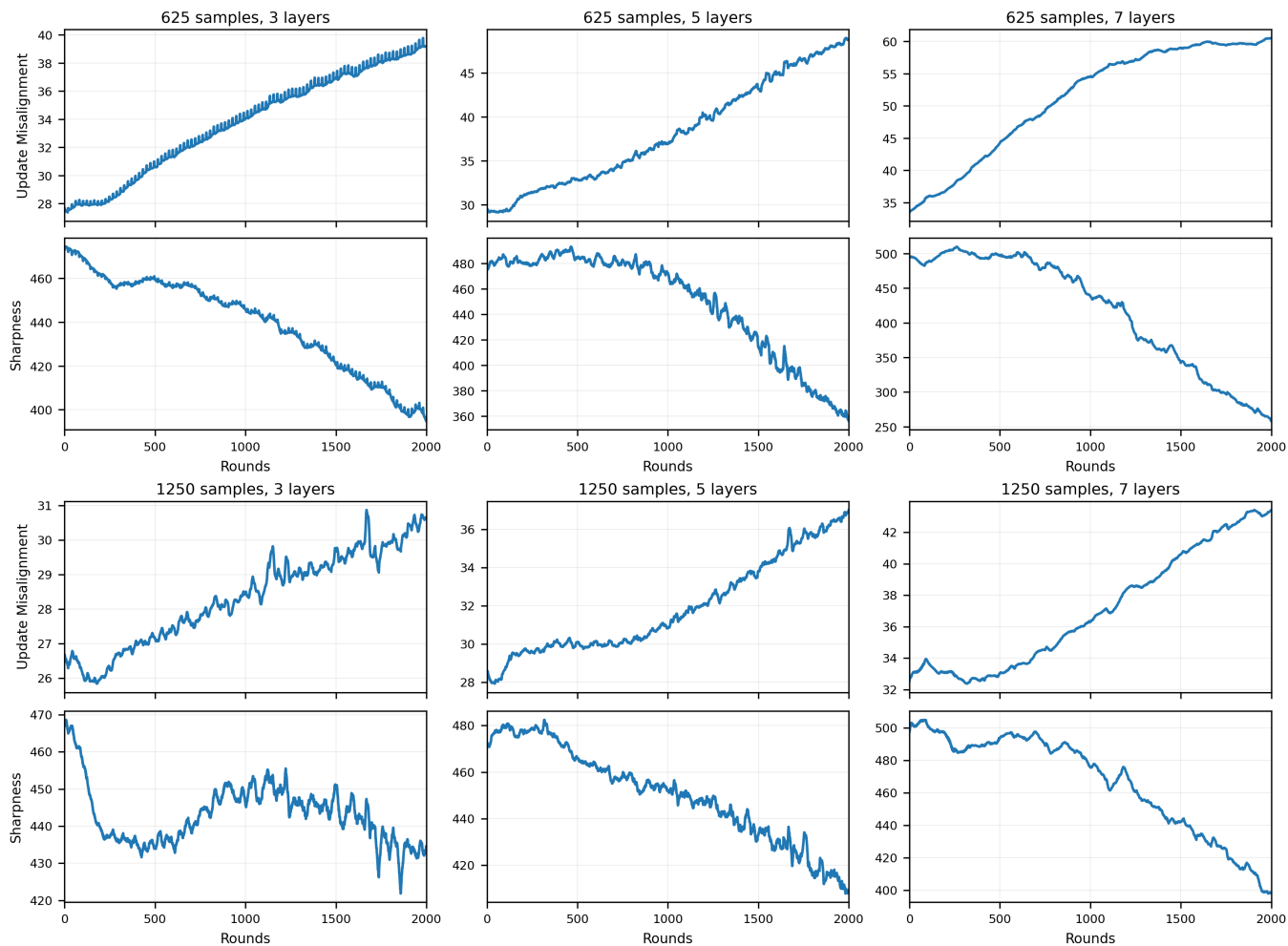
Figure 9: Update misalignment and local sharpness values over FedAvg trajectories for Table 2. For FedAvg, update misalignment and sharpness are empirically disassociated.
