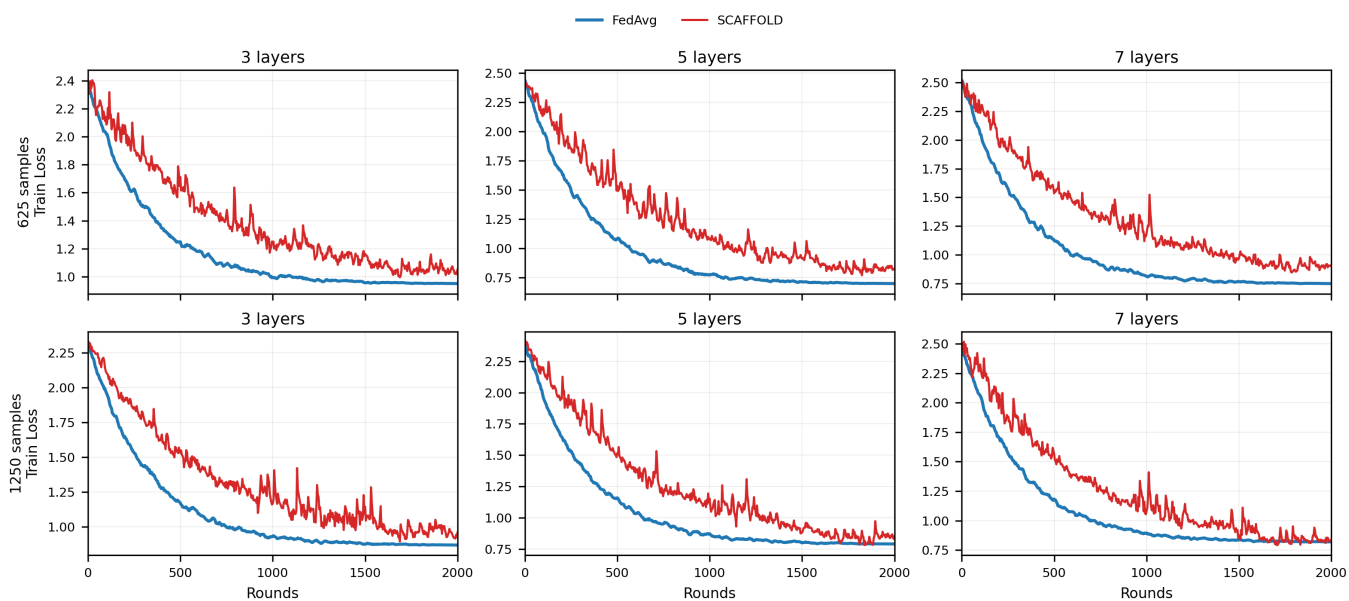
Figure 10: Loss curves for 2 with a CIFAR dataset for both SCAFFOLD and FedAvg for CNNs of depth 3, 5, and 7 and dataset sizes of 625 and 1250. FedAvg consistently attains lower loss and converges faster, with less instability in loss.
