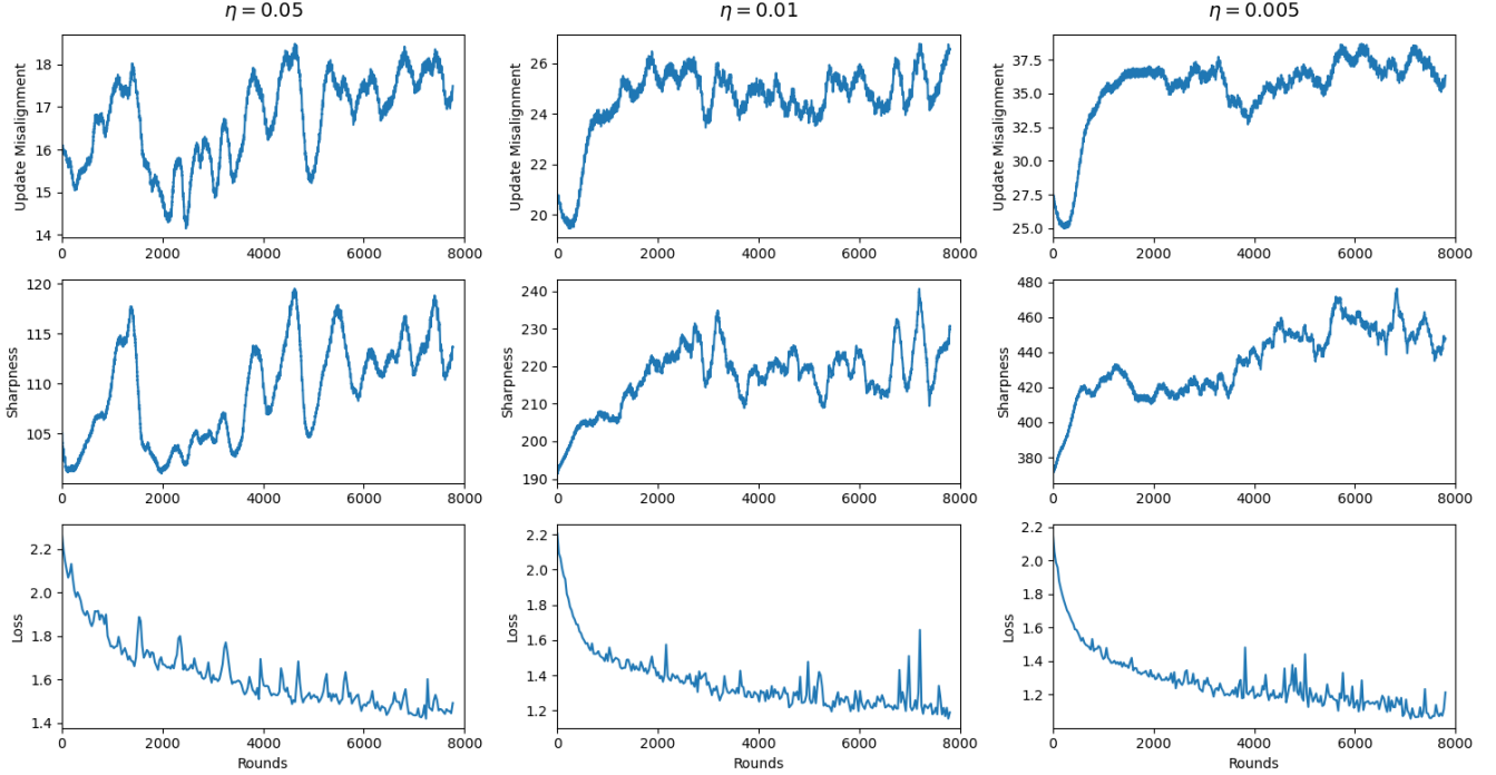
Figure 3: Update misalignment (top), local sharpness (middle), and training loss (bottom) of SCAFFOLD with various learning rates on CIFAR-10 using a shallow CNN architecture. Update misalignment and sharpness are clearly correlated, implying that sharpness causes instability and drift in SCAFFOLD.
