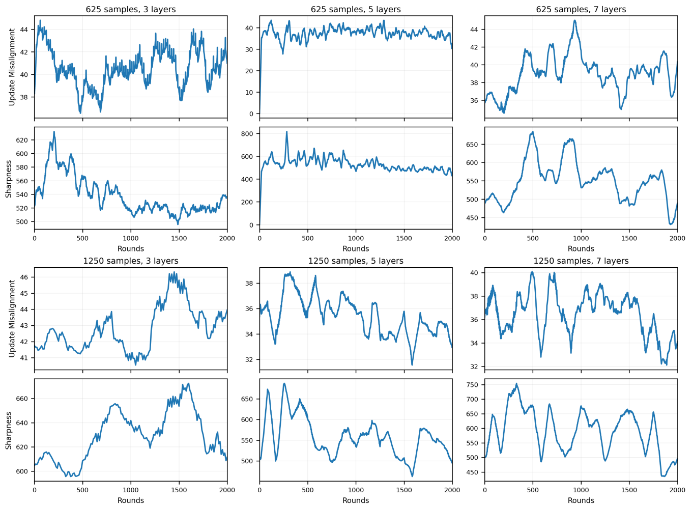
Figure 8: Update misalignment and local sharpness values over SCAFFOLD trajectories for Table 2. Update misalignment and sharpness stay highly correlated across different architectures and dataset sizes for SCAFFOLD.
