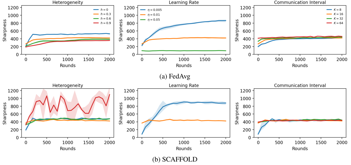
Figure 2: Sharpness of local objectives with varying heterogeneity, learning rate, and communication interval (three-layer CNN, CIFAR-10 dataset), averaged over three random seeds. Error bars denote min and max values among 3 samples. Note that SCAFFOLD training with a learning rate of 0.05 diverged, so we omit the corresponding curve. Federated algorithms only have a clear inverse relation to learning rate, with minimal relation to heterogeneity or communication interval except for SCAFFOLD in the case of very high heterogeneity.
