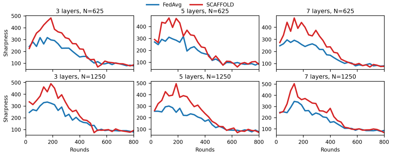
Figure 7: MNIST local sharpness values during training for many CNN layer depths and dataset sizes, as referenced in 2. For MNIST, sharpness rises initially, and then gradually decreases as the network converges to 0 loss.
