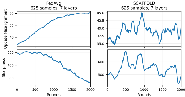
Figure 4: Update misalignment and sharpness for FedAvg and SCAFFOLD on CIFAR-10 with 625 samples and 7 layers. The peaks and valleys of SCAFFOLD’s update misalignment closely track that of the sharpness, unlike FedAvg.
