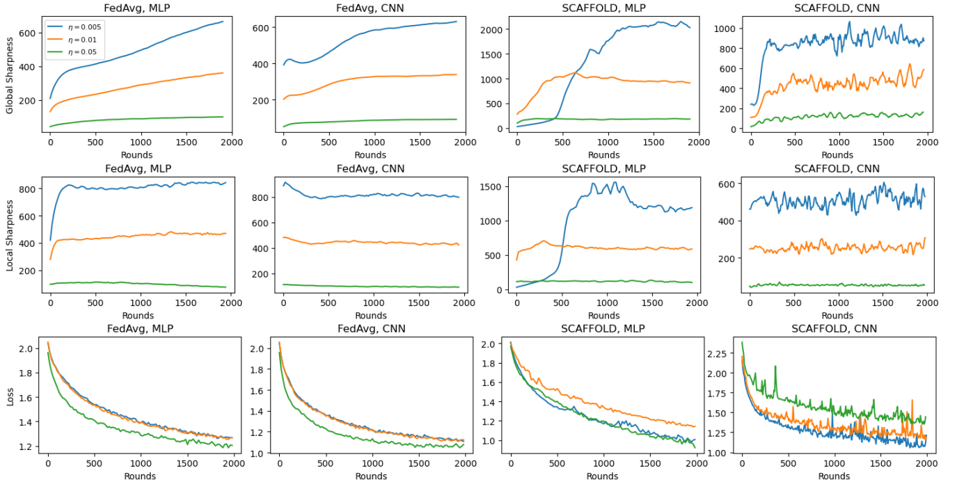
Figure 1: Sharpness and loss trajectories for FedAvg (left) and SCAFFOLD (right) on CIFAR-10 with MLPs and CNNs (three layers). We measure sharpness of the global objective (top), sharpness of the local objectives (middle), and training loss (bottom). Both SCAFFOLD and FedAvg experience progressive sharpening in terms of the global sharpness and the local sharpness.
