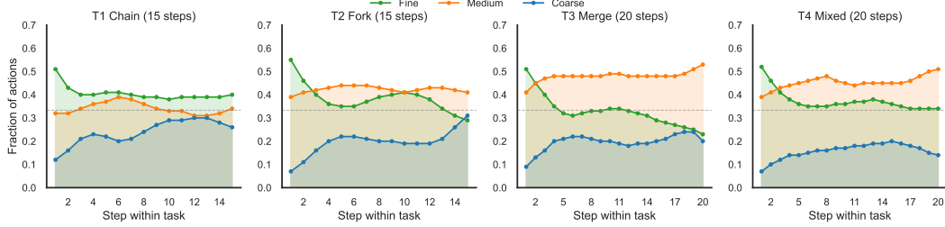
Figure 7: Granularity use by task and step. Across the four tasks, medium use increases while coarse use decreases. Within a task, fine use decreases and coarse use increases from the first to the second half of exploration.
