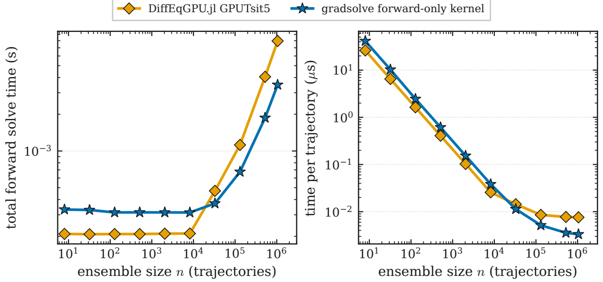
Figure 5: Forward solve time, total (left) and per trajectory (right), against ensemble size on the Lorenz system (double precision, matched tolerance \tau_{\text{rel}} = 1 \times 10^{-6} , \tau_{\text{abs}} = 1 \times 10^{-9} ). Per-trajectory cost falls with ensemble size as launch overhead spreads over more trajectories. The plotted DiffEqGPU.jl sweep ran on a different A100 and is shown only for the shape of its scaling; the forward-only kernel was swept on an A100-SXM4 at the same tolerances, and the like-for-like same-card comparison, in which the forward-only kernel is 2.8\times faster, is given in the text.
