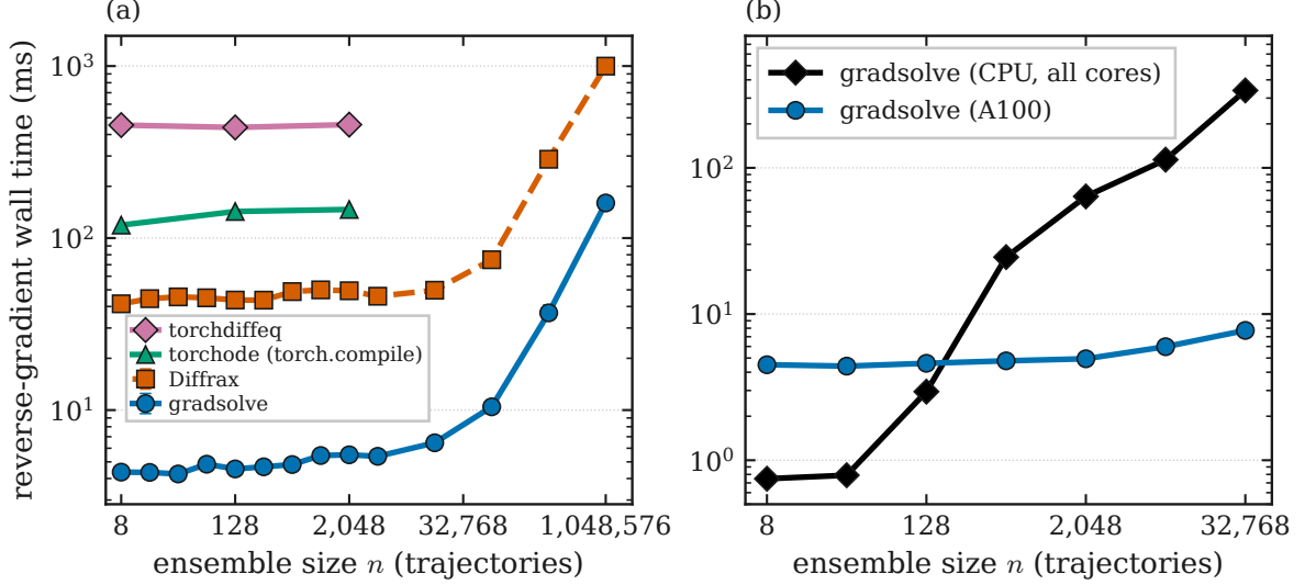
Figure 6: Reverse-mode gradient cost against ensemble size on the Lorenz system at matched achieved accuracy (double precision). (a) On the A100, the record-and-replay adjoint computes the gradient 9.0\text{--}10.7\times faster than Diffrax’s checkpointed adjoint across the sweep of ensemble sizes from n = 8 to 2048 and 6.2\text{--}8.5\times faster out to n = 1\,048\,576 , and one to two orders of magnitude faster than torchode (under torch.compile ) and torchdiffeq, shown at representative sizes and timed on a second A100 of the same class. The Diffrax and record-and-replay points carry an up-whisker to the slowest of their three timed calls, mostly narrower than the marker, the run-to-run spread being 12.6% at worst (Appendix B.3). (b) The same record-and-replay gradient on the CPU of the machine hosting the A100 and on the A100 itself: the CPU is faster for small ensembles, the curves cross between n = 128 and n = 512 , and the GPU leads from there upward.
