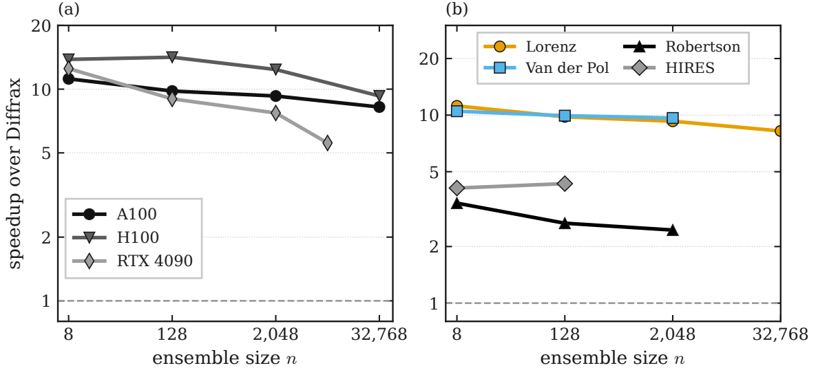
Figure 8: Matched-accuracy gradient speedup over Difffrax against ensemble size (double precision). (a) Lorenz on three GPU generations: the advantage spans 5.6\text{--}14.1\times on the three cards and declines with ensemble size on each, remaining above the parity line (dashed). (b) Four systems of the suite on the A100: the non-stiff Lorenz and Van der Pol systems and the stiff Robertson and HIRES systems, all above parity at the accuracy swept here. HIRES differentiates with respect to its initial state, since it has no free parameter.
