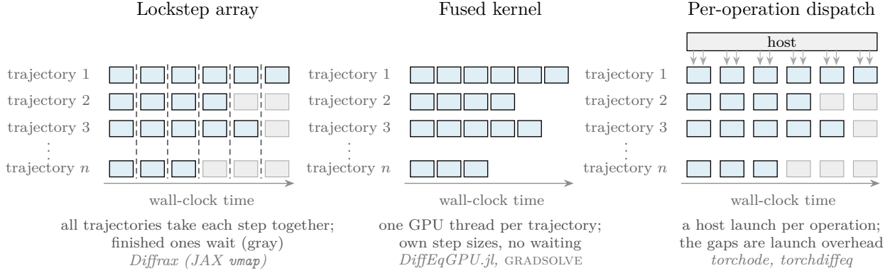
Figure 1: The same ensemble of n trajectories under the three GPU execution designs, showing the first three trajectories, needing six, four, and five accepted steps, and the last, the n -th, needing three. Each row is one trajectory. Each block is one accepted step of the adaptive loop of Section 2.1: the Runge–Kutta stage evaluations of the right-hand side of the ODE, followed by the error test and the controller decision. Block width is uniform and does not represent step size, and rejected trials are not drawn. Horizontal position tracks wall-clock time in every panel, along the bottom arrow; the white gaps between steps in the right panel are the launch overhead, drawn as blank space. Left: a lockstep array program advances all trajectories together, one loop iteration per dashed line, in which every trajectory takes one trial step of its own size, so trajectories that finish early wait through the remaining iterations (gray). Center: a fused kernel gives each trajectory its own thread, with its own step sizes, so each row ends when its work ends. Right: per-operation dispatch launches each operation of each step (stage evaluations, error norm, controller update) as its own kernel from the host (the CPU that drives the GPU); two launch arrows are drawn per step; finished trajectories wait (gray) as in the left panel, and the white gaps between steps are the launch overhead, stretching the same work over more wall-clock time. GRADSOLVE builds on the fused design.
