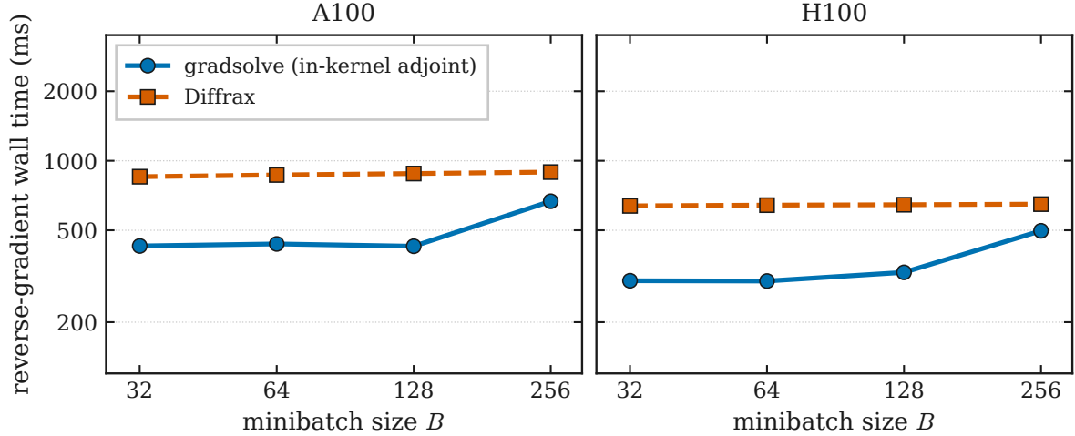
Figure 11: Per-step gradient time against minibatch size B for the Robertson system with a neural reaction term, on the A100 and the H100, with DiffraX’s tolerance fixed at the value matching the replay’s achieved error. GRADSOLVE’s in-kernel adjoint is faster at every minibatch size measured, by a margin that is about 2\times at the smaller batch sizes and narrows at B = 256 .
