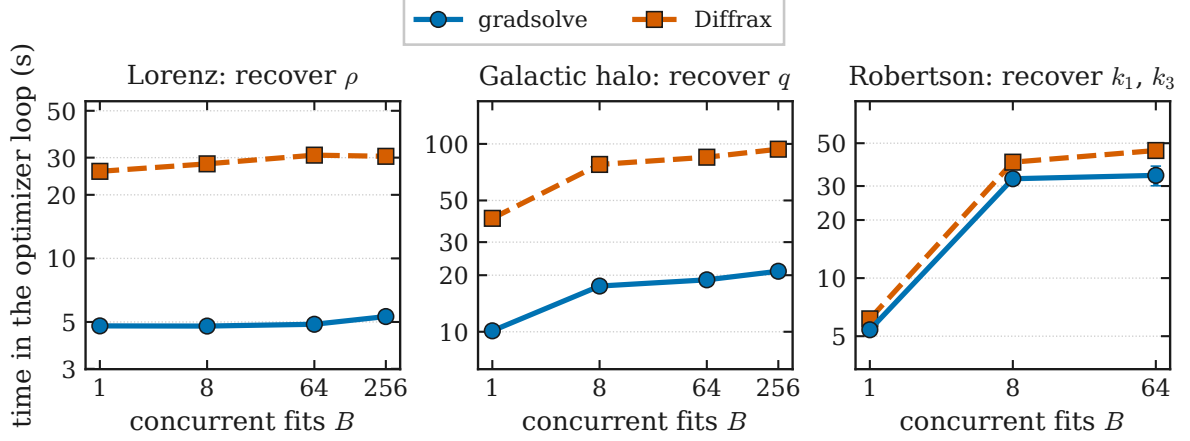
Figure 10: Time in the optimizer loop against the number of concurrent fits B at matched accuracy (A100), recovering the Lorenz Rayleigh parameter \rho (left), the galactic halo flattening q (center), and the Robertson rate constants (right). The lower gradient cost translates into a faster fit in every panel. Error bars are the standard deviation over the timed repetitions; the run-to-run spread is under about 3% at almost every point (up to about 12% at the noisiest), so the bars mostly fall within the markers. The Robertson B = 256 point is absent because neither engine reached the loss tolerance there.
