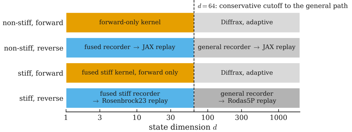
Figure 4: Engine dispatch. Each row is one kind of request (non-stiff or stiff, forward solve or gradient) and the horizontal axis is the state dimension d ; the boxes name the engine of Table 1 the router selects. Gold marks the two fused forward-only kernels, blue the fused recorder followed by the differentiated replay, and gray the general path, taken by every right-hand side without a fused kernel and by all states beyond d = 64 .
