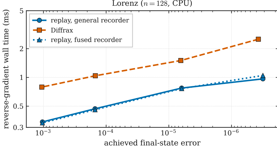
Figure 12: Per-gradient cost against achieved final-state error on the Lorenz system ( n = 128 , double precision, CPU). Both GRADSOLVE curves run the same differentiated JAX replay and differ only in how the mesh was recorded, by the general recorder or by the fused recorder; recording is excluded from the per-gradient time. The two therefore track each other closely, and both sit below Diffrax’s checkpointed adjoint across the tolerance range. The gap to Diffrax thus measures the effect of differentiating a fixed-step replay rather than of any GPU kernel.
