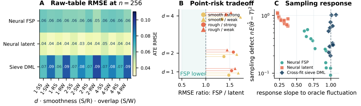
Figure 8: Neural FSP on unbinned continuous covariates. The 12 mechanisms use 400 common tables each at n = 256 ; neural metrics average three checkpoints. Panel A resolves dimension, smoothness and overlap; B shows the point-risk cost of moving toward the efficient sampling response; C compares native defect with response slope. Latent supervision has lower point RMSE, whereas FSP recovers more efficient fluctuation.
