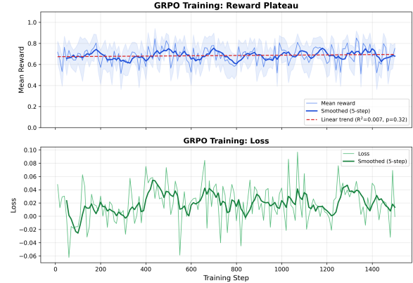
Figure 5: GRPO training reward over 1500 steps. The reward oscillates without a clear upward trend ( R^2 = 0.007 , p = 0.32 ), indicating early reward saturation.
