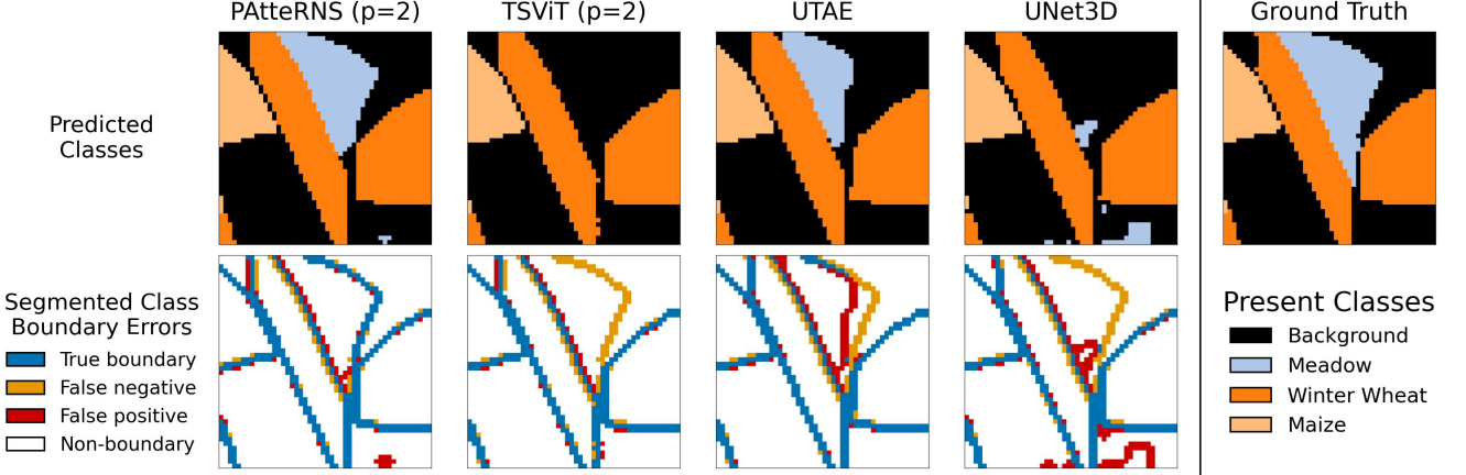
Figure 6: An illustration of PATteRNS’ segmentation capabilities against comparison models. Our model is shown here to combine precise boundaries with full recall of present classes in the ground truth labels of a tile from MTLCC-48.
