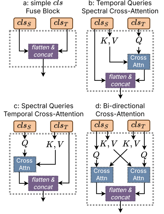
Figure 4: The compared Fuse Block structures for the \text{cls} token fusion following our parallel spectral and temporal transformer branches. The outputs of these fuse blocks are passed onwards to the spatial embedding process, and then the spatial transformer.
