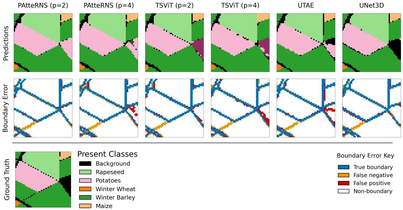
Figure C.8: Class segmentation outputs, and boundary error maps, for all models on an example tile from MTLCC-48.
