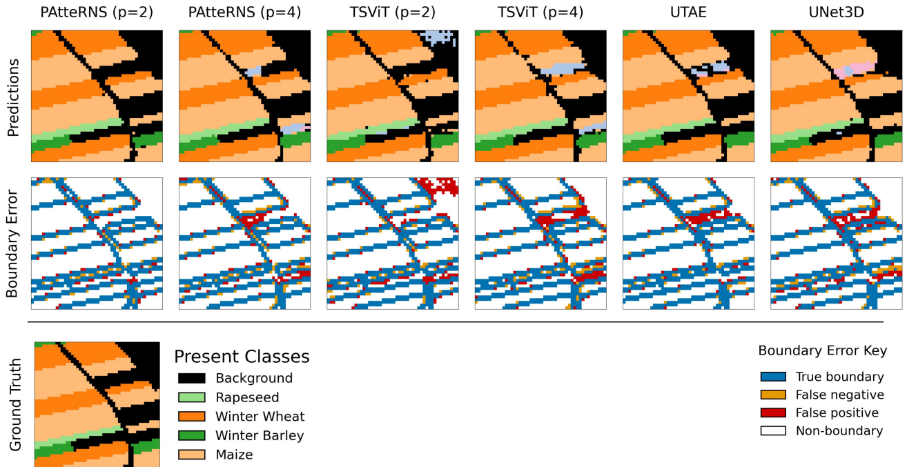
Figure C.9: Class segmentation outputs, and boundary error maps, for all models on an example tile from MTLCC-48.
