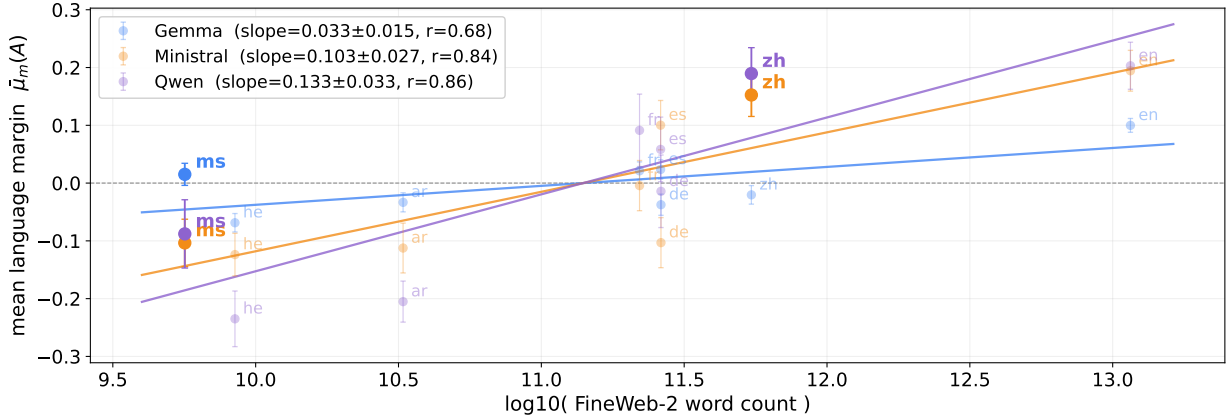
(b) Mean language margin against web-text availability, measured by \log_{10} FineWeb-2 word count, with English estimated from FineWeb.
