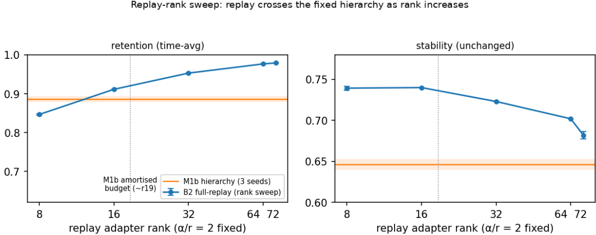
Figure 3: Replay-rank sweep used as a falsification control. Consistent with prior LoRA-memory work, replay retention rises and saturates with rank; the distinctive result here is that replay crosses the fixed hierarchy. Stability is flat to rank 16 and then falls. The hierarchy’s 3-seed band is shown for comparison.
