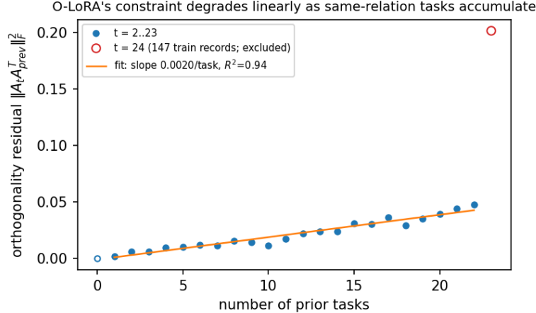
Figure 4: O-LoRA’s orthogonality residual against prior-task count. The residual grows approximately linearly through t=23 ( R^2=0.94 ); the final month (open marker) contains fewer training records and is excluded from the fit.
