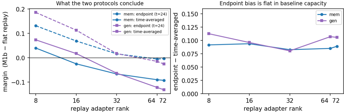
Figure 2: For the fixed hierarchy, replay rank changes the method-comparison margin. Left: endpoint and time-averaged hierarchy-minus-replay margins versus replay rank. Right: their difference, the endpoint bias. Replay rank shifts the level, while boundary-aligned timing adds a similar positive bias across the tested ranks.
