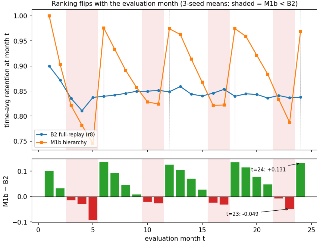
Figure 1: The consolidation sawtooth and the months in which the ranking flips (3-seed means). Shaded months are those where flat replay leads; dotted lines mark consolidation boundaries. The two candidate endpoints t=23 and t=24 give opposite answers.
