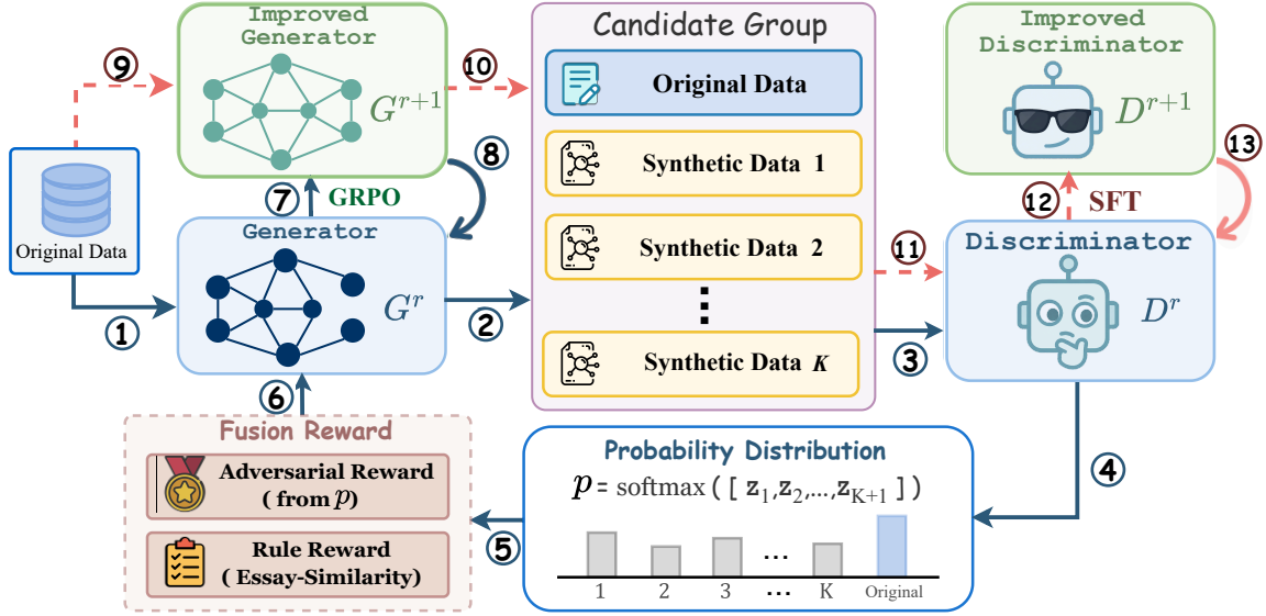
Figure 1: Overview of the proposed framework. The framework consists of two iterative stages: generator optimization (①–⑧) and discriminator refinement (⑨–⑬). Through alternating adversarial training, the generator and discriminator progressively improve together.
