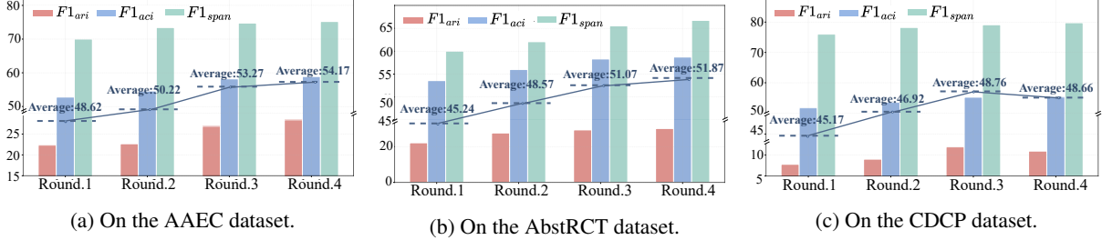
Figure 2: Performance comparison of different rounds. Here, we use the ST model for AM.
