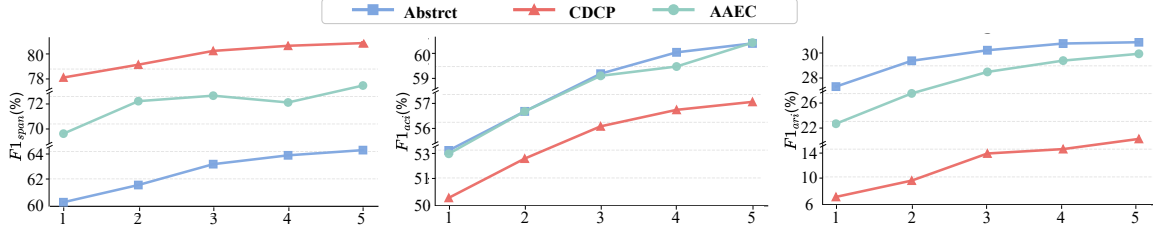
Figure 3: Performance comparison under different numbers of synthetic samples ( K ) using the ST model for AM.
