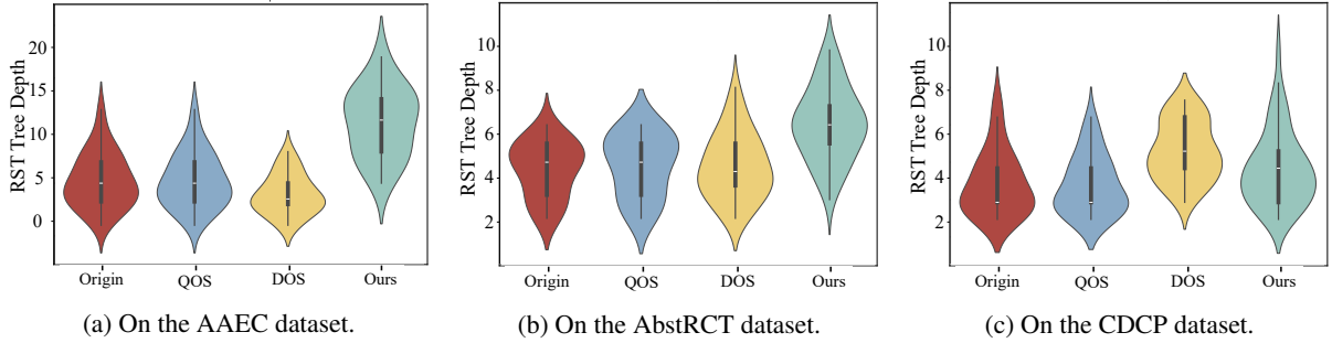
Figure 5: RST tree depth distributions of different argument data under the full-data setting.
