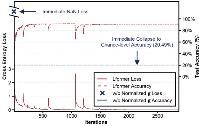
Fig. 7: Optimization dynamics during the stabilization ablation on the PTS-C benchmark. The left and right vertical axes track training loss convergence (solid curves) and out-of-sample test accuracy (dashed curves), respectively.
