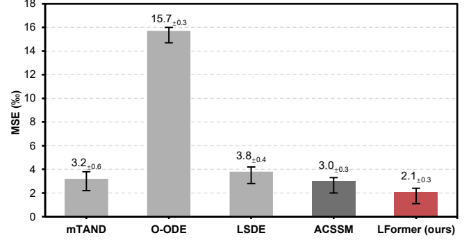
(b) PTS-R MSE on the PDL dataset
