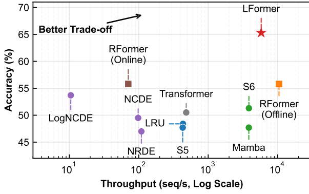
(a) Pareto Frontier on the MI Dataset
