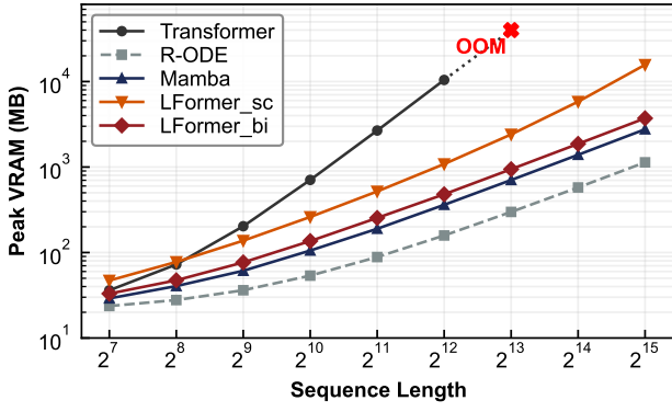
(a) Peak GPU Memory Usage
