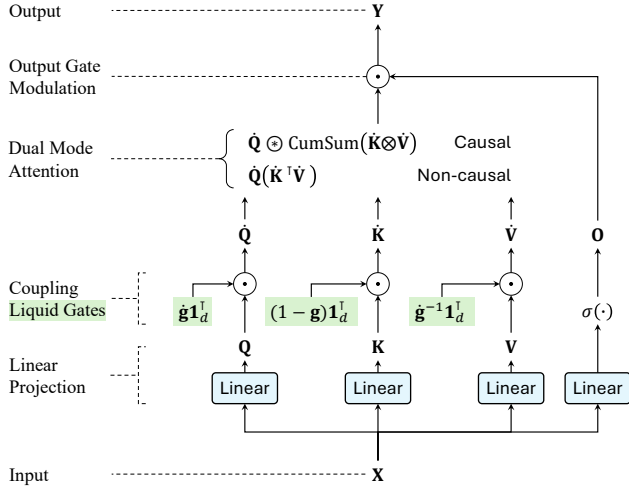
Fig. 2: Parallel LGA pipeline. The input representation \mathbf{X} is first projected and scaled by vectorized liquid gates to embed continuous-time gating dynamics, yielding modulated representations. The dual mode attention block then executes either a causal prefix scan or a global matrix multiplication with linear complexity. The output gate modulates the aggregated state to produce the final representation. \odot , \otimes , and \oplus denote the element-wise product, row-wise vector-matrix multiplication, and row-wise matrix outer product, respectively. \text{CumSum}(\cdot) computes the cumulative sum along the temporal dimension.
