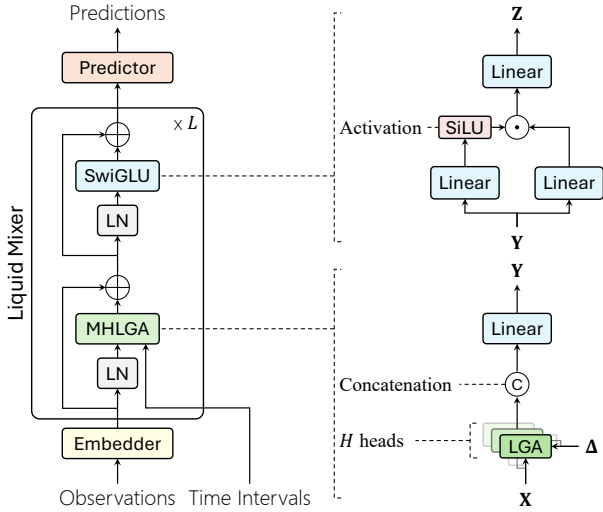
Fig. 3: LFormer architecture. The left block depicts the macro design, where L stacked Liquid Mixers connect a task-specific Embedder and Predictor. The right panels detail the MHLGA (bottom) and SwiGLU (upper) workflows.
