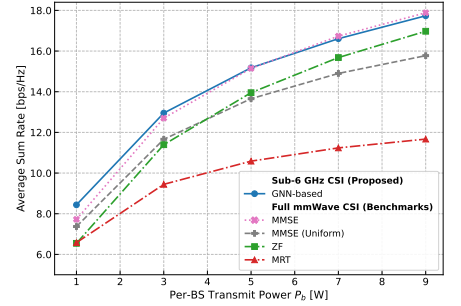
Fig. 3. Sum-rate versus per-BS transmit power P_b for the proposed GNN-based beamformer and benchmark beamformers.
