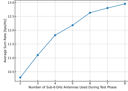
Fig. 2. Sum-rate of the GNN-based framework versus the number of available sub-6 GHz antennas at inference for P_b = 3 W.
