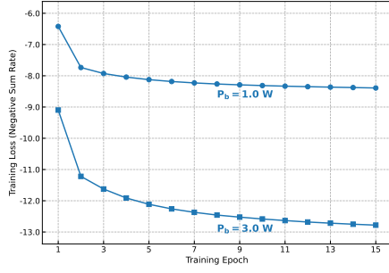
Fig. 1. Training loss convergence of the proposed framework for two representative per-BS transmit powers, P_b \in \{1, 3\} W.
