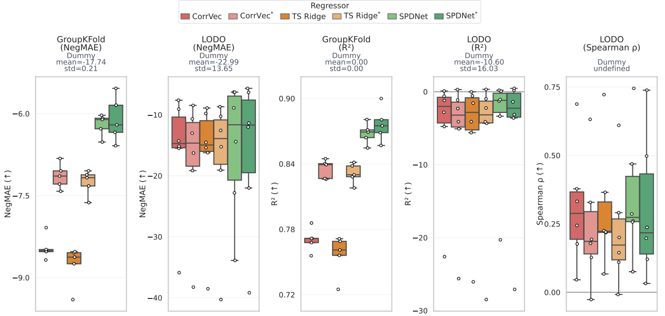
Figure 4: Across-dataset prediction benchmark on the pooled sample from COBRE, ADNIDOD, Cam-CAN, ABIDE, OASIS-3, and ADNI. The five panels report GroupKFold negative MAE, LODO negative MAE, GroupKFold R^2 , LODO R^2 , and LODO Spearman \rho . Boxplots compare CorrVec, Tangent-Space Ridge (TS Ridge), and SPDNet, each in original form and after harmonization. A superscript * denotes the harmonized version of a method. Dummy scores are shown as panel annotations because the Dummy regressor is a constant-prediction reference; its Spearman \rho is undefined. Each LODO point corresponds to one held-out dataset.
