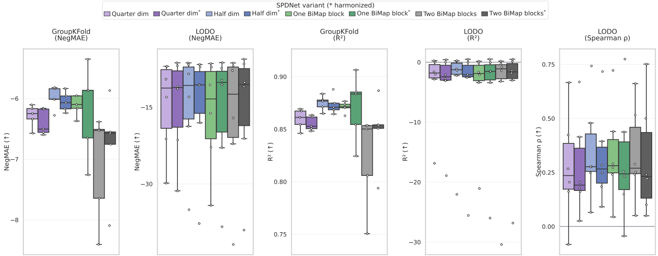
Figure 5: SPDNet configuration ablation under pooled GroupKFold and LODO evaluation. The five panels report GroupKFold negative MAE, LODO negative MAE, GroupKFold R^2 , LODO R^2 , and LODO Spearman \rho . Boxplots compare four SPDNet variants: quarter dimension, half dimension, one BiMap block, and two BiMap blocks, each in original form and after harmonization. A superscript * denotes the harmonized version of a variant. Overall, no single SPDNet configuration is consistently best across these diagnostics.
