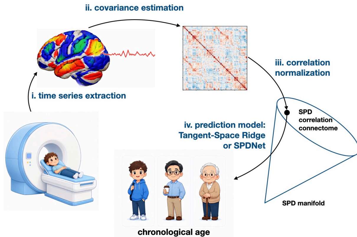
Figure 1: Overview of the rs-fMRI regression pipeline. Starting from each scan included in the analysis, we (i) extract regional time series, (ii) estimate a regularized covariance matrix, and (iii) normalize it to a correlation matrix. The resulting SPD correlation connectome is then passed to (iv) the prediction model, Tangent-Space Ridge or SPDNet, to predict chronological age.
