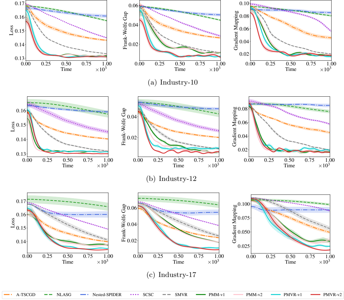
Figure 3: Results for mean-deviation risk-averse portfolio optimization.
