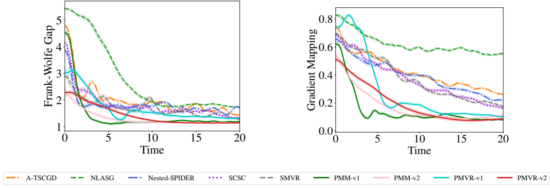
Figure 1: Results for matrix optimization with low-rank constraints.
