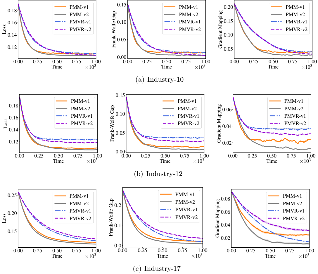
Figure 5: Results for mean-variance risk-averse portfolio optimization.
