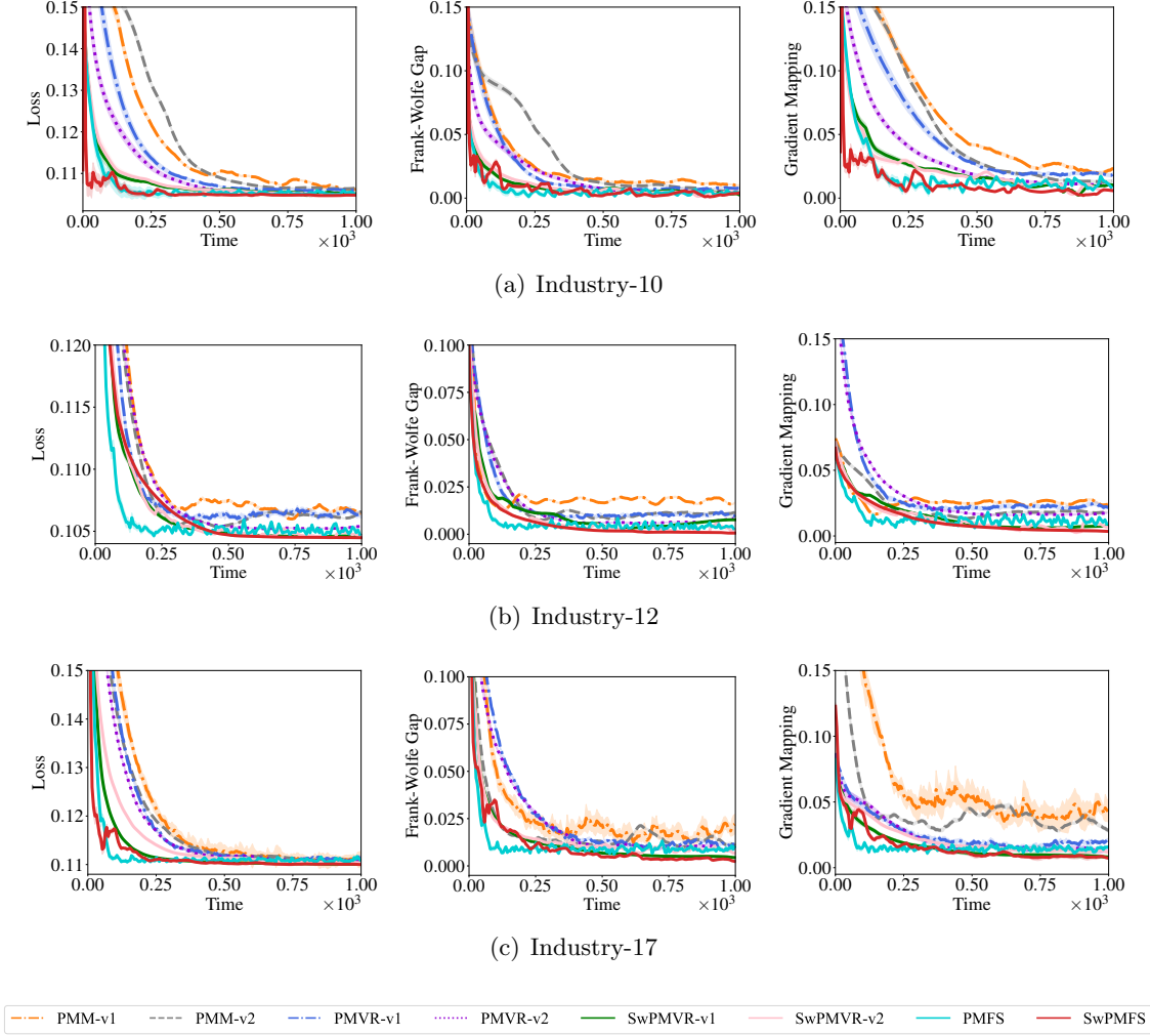
Figure 4: Results for mean-variance risk-averse portfolio optimization.
