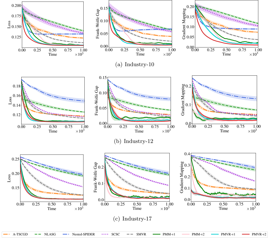
Figure 2: Results for mean-variance risk-averse portfolio optimization.
