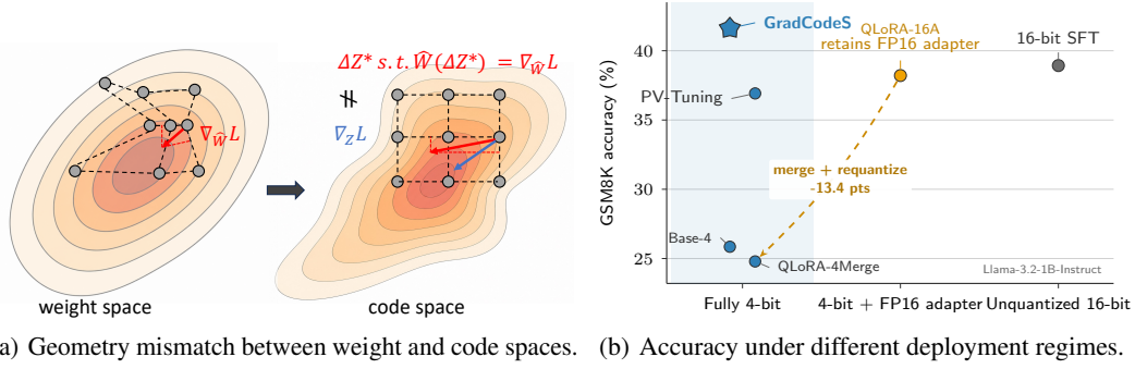
Figure 1: Motivation for deployment-faithful code-space optimization. (a) Group scales and non-uniform codebook gaps distort local geometry, so a weight gradient does not identify the best discrete code move. (b) In the Llama-3.2-1B GSM8K example, continuous adaptation either retains an FP16 adapter or loses 13.4 points after QLoRA requantization; GradCodeS improves the fully 4-bit result while retaining a deployable checkpoint.
