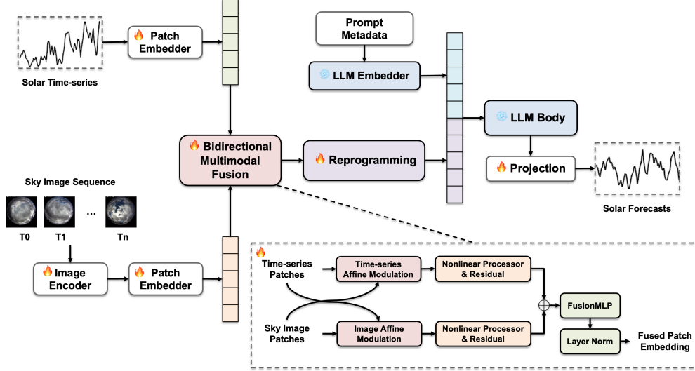
Figure 1: The overall architecture of SolCloudLLM. Historical solar time-series and aligned sky images are encoded into patch tokens and integrated via a bidirectional multimodal fusion module. The fused representations then undergo patch reprogramming, followed by a frozen LLM backbone and a linear projection head to generate the final forecast. The fire and snowflake icons denote trainable and frozen components, respectively.
