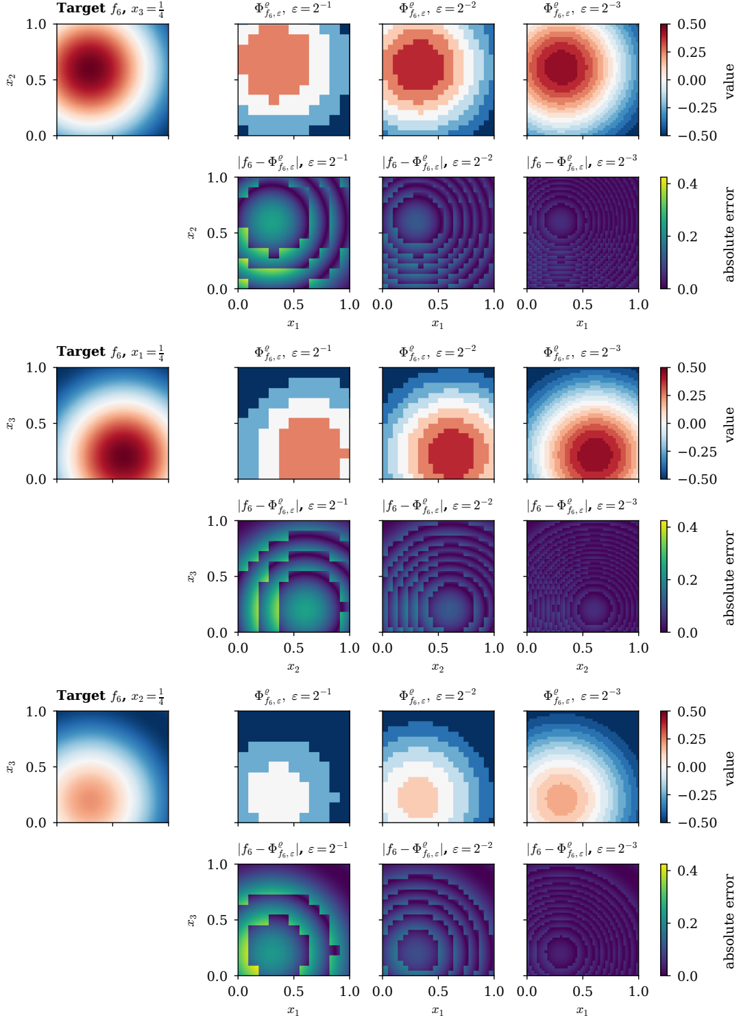
Figure 12: Numerical verification of Theorem 3.1 for the approximation of the 3D function f_6 by the four-neuron network \Phi_{f_6, \varepsilon}^\theta . The sections and panels are arranged as in Figure 11, with \varepsilon = 2^{-1}, 2^{-2}, 2^{-3} and M = 11, 22, 44 .
