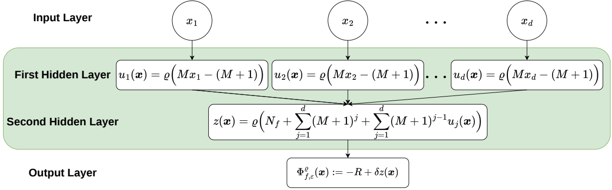
Figure 3: Architecture of the network \Phi_{f,\varepsilon}^\varrho in Theorem 3.1. The d neurons in the first hidden layer quantize the input coordinates, whose weighted combination forms the cell address r(\mathbf{x}) ; the neuron in the second hidden layer decodes the corresponding quantized value from the stored integer N_f . The network has d + 1 hidden neurons in total.
