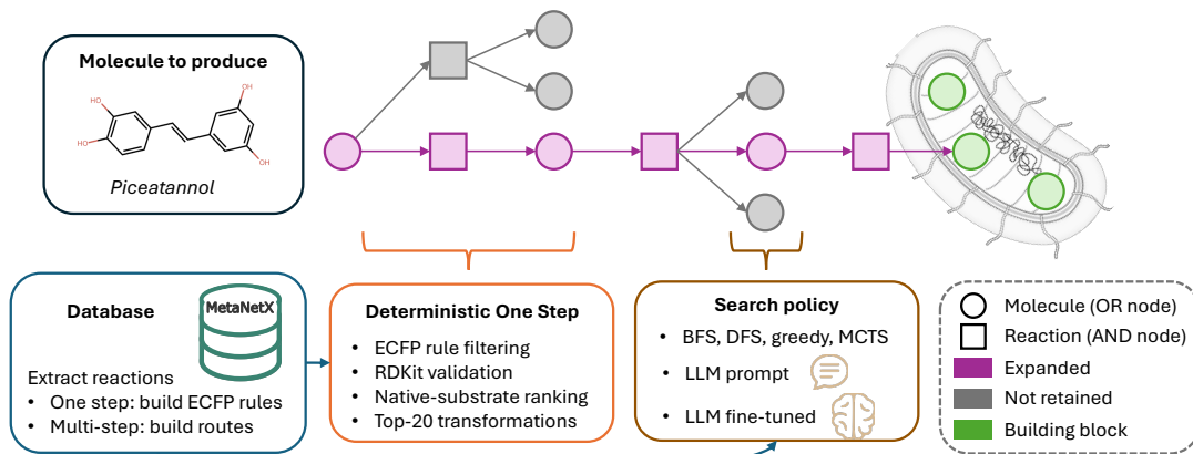
Figure 1: Overview of the agentic retrosynthesis framework. A target molecule is expanded through a deterministic MetaNetX-derived one-step engine, while the search policy selects which frontier molecule to expand next. The search proceeds toward the E. coli terminal metabolite set.
