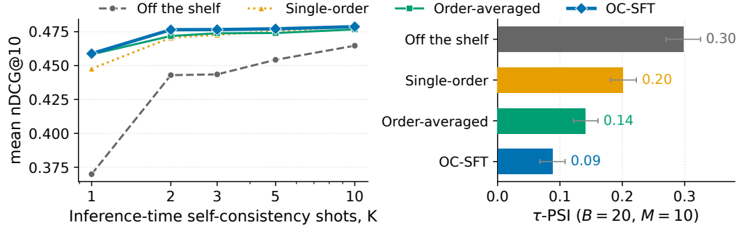
Figure 6: OC-SFT at K = 1 is within 0.006 nDCG@10 of the off-the-shelf K = 10 ensemble. Left: nDCG@10 against self-consistency permutations K , higher is better. Right: single-pass \tau -PSI at B = 20 for off the shelf, single-order distillation, order-averaged distillation and OC-SFT, evaluated over M = 10 random permutations; lower is better.
