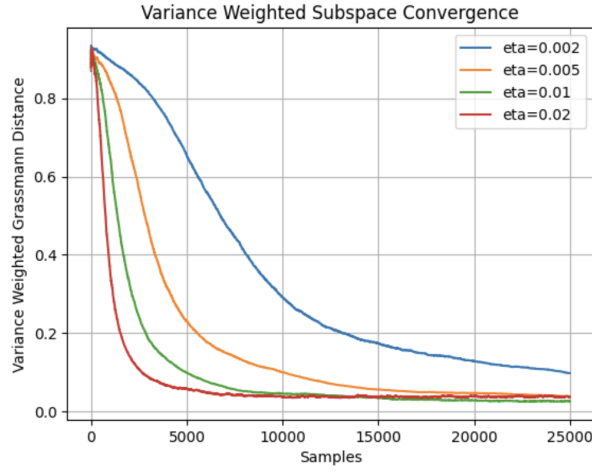
Fig. 1: (a) Variance-weighted subspace distance and (b) cosine similarity of the first eigenvector, for increasing learning rate \eta . Larger \eta yields faster convergence at the cost of increased noise.
