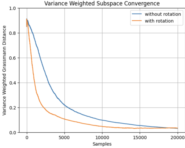
Fig. 2: Variance-weighted subspace distance versus number of samples, with and without the rotation-based update enabled. Enabling rotation yields substantially faster convergence.
