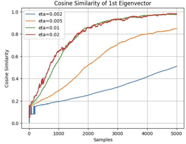
Fig. 1: (a) Variance-weighted subspace distance and (b) cosine similarity of the first eigenvector, for increasing learning rate \eta . Larger \eta yields faster convergence at the cost of increased noise.
