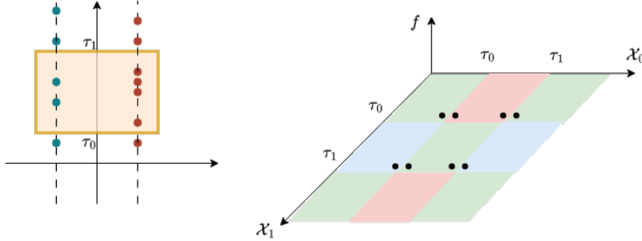
Figure 18: Illustration of the dual star number for the dual class relative to \mathcal{H}_{\mathbb{R}^2}^{\text{rec}} .
