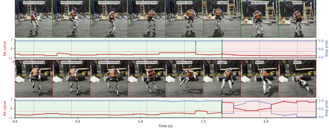
Figure 1: Safe-stop accurately predicts the stoppability of the robot. Top: When the estimates lie in a recoverable range with low reach-avoidance value \hat{V}_\psi and high stop-probability estimate \hat{P}_\phi , triggering stop policy leads to a stable halt immediately. Bottom: When the estimates lie in an unrecoverable range, the stop policy leads to a fall as predicted.
