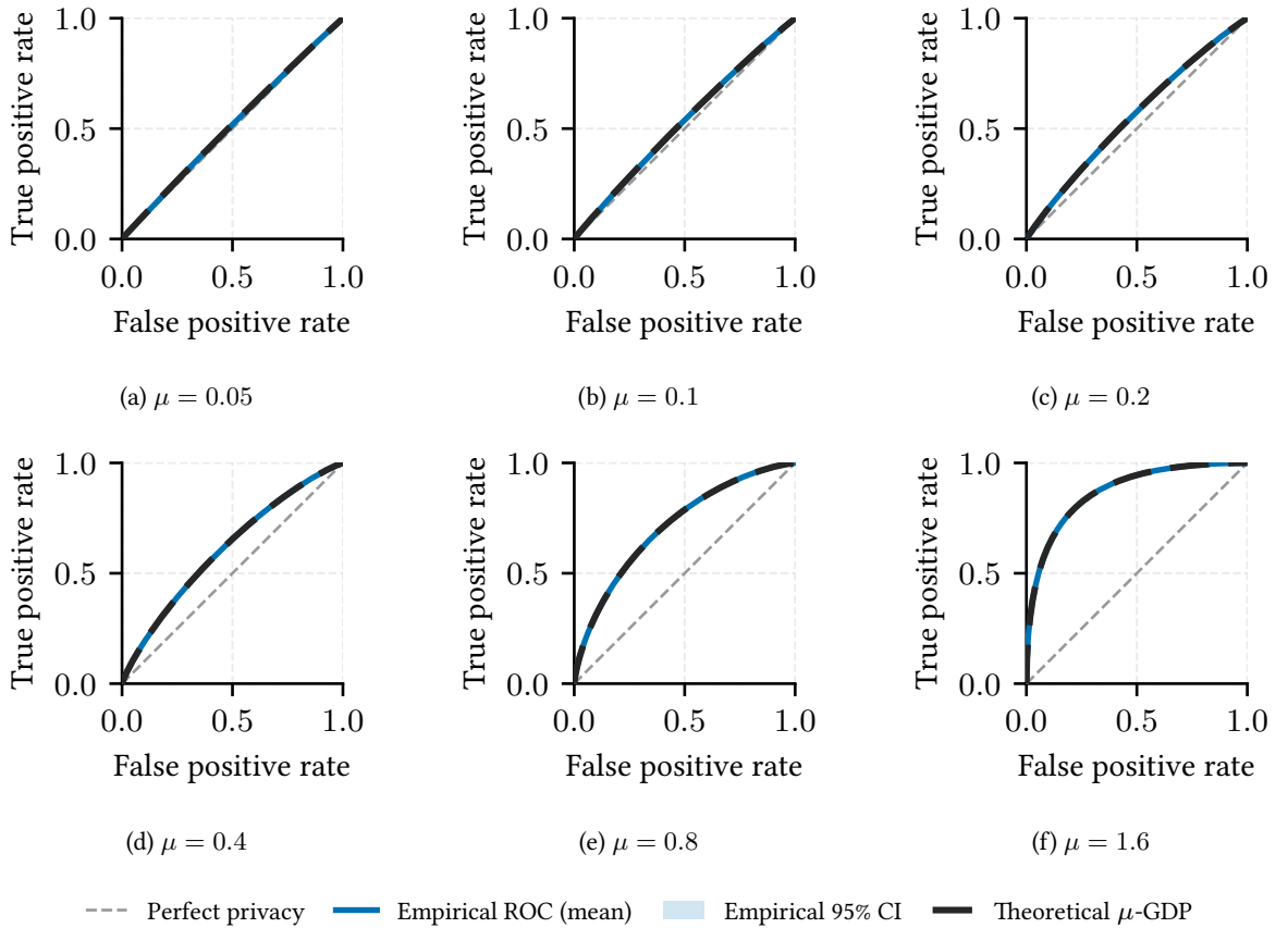
Figure S4: Empirical audit of the DP-MHCA mechanism across privacy levels. For each \mu , the audit optimises a pair of adjacent token sets to maximise the pre-noise output difference and then estimates the trade-off curve from repeated samples of the privatised outputs, using 10 repeated audit runs; shaded bands show pointwise bootstrap 95% CIs over those runs. The resulting curves are compared against the strongest likelihood-ratio attack with access to the unnoised means and the calibrated noise standard deviation. The observed behaviour is consistent with the intended privacy calibration across the full range of \mu .
