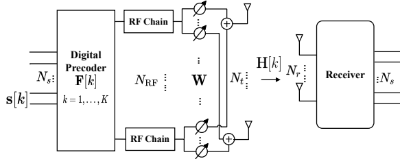
Fig. 1: Block diagram of a single-user MIMO-OFDM system with hybrid beamforming at the BS.
