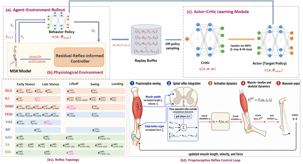
Figure 1: Overview of the proposed Residual-Reflex RL framework. (a) The rollout policy maps the musculoskeletal state \mathbf{s}_t to a four-dimensional residual action \mathbf{a}_t and collects transitions (\mathbf{s}_t, \mathbf{a}_t, r_t, \mathbf{s}_{t+1}) . (b) The physiological environment combines the muscle-driven character with a phase-dependent residual-reflex-informed controller. In the enlarged lower row, panel (b1) on the left shows the sparse phase-dependent reflex topology, while panel (b2) on the right shows the proprioceptive control loop from muscle sensing to stimulation, activation, muscle-tendon force, skeletal motion, and updated sensory feedback. Magenta entries in (b1) denote the four reflex parameters modulated by \mathbf{a}_t . Superscripts (all), (st), and (sw) identify parameters shared across all five phases, Early Stance–Late Stance, and Liftoff–Swing–Landing, respectively. The notation i \leftarrow j indicates that feedback from source muscle j modulates target muscle i ; entries without a source are self-feedback pathways. (c) The collected transitions are stored in \mathcal{D} ; the critic q(\mathbf{s}, \mathbf{a}; \omega) evaluates candidate actions and MPO updates the rollout policy from \pi(\mathbf{s}; \theta_{\text{now}}) to \pi(\mathbf{s}; \theta_{\text{new}}) .
