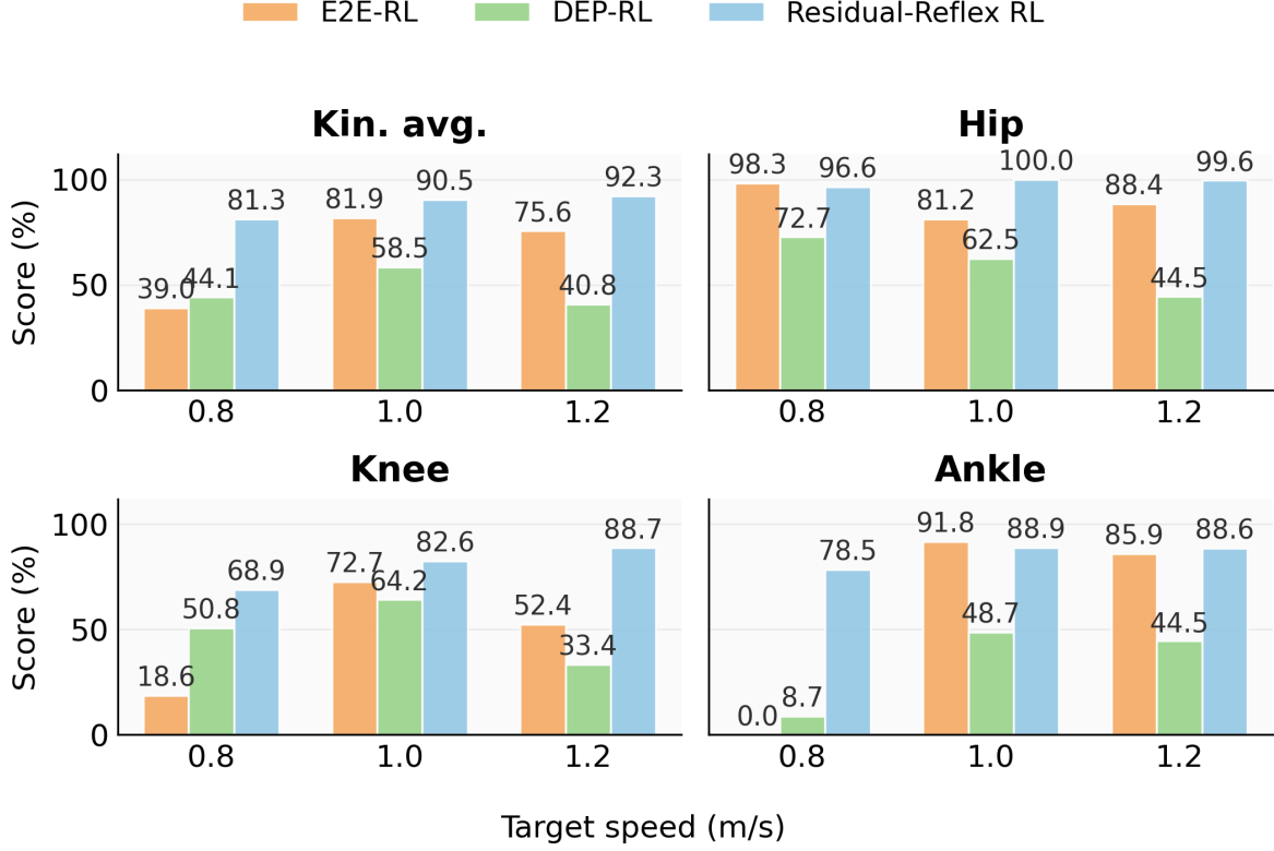
Figure 3: Human-reference kinematic gait scores across target speeds. Numeric labels indicate the score of each bar. The Residual-Reflex RL controller achieves the highest kinematic-average score and especially improves knee and ankle components.
