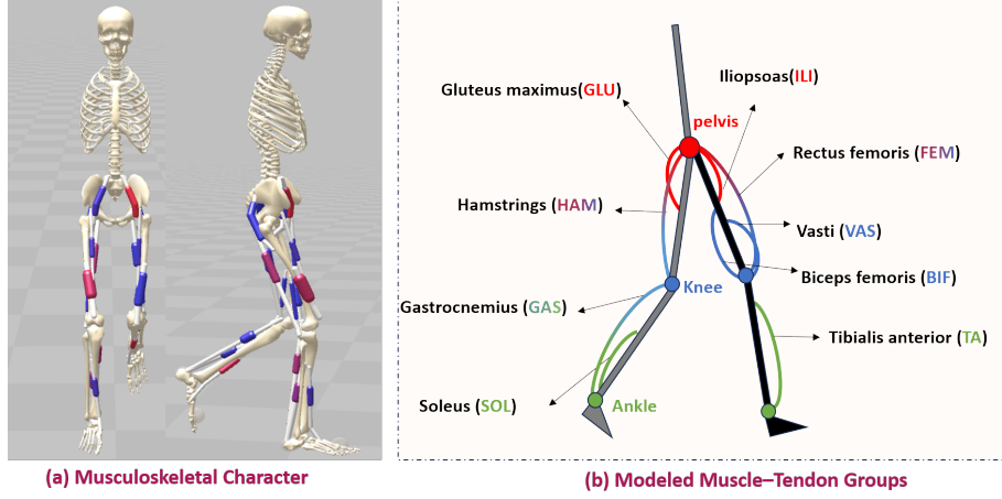
Figure 2: Muscle-driven character model. (a) Front and sagittal views of the H0918v2j character used in the experiments. (b) Schematic arrangement and primary joint functions of the nine bilateral muscle–tendon groups. The complete character is actuated by 18 Hill-type muscle–tendon units, with one instance of each modeled group on each leg.
