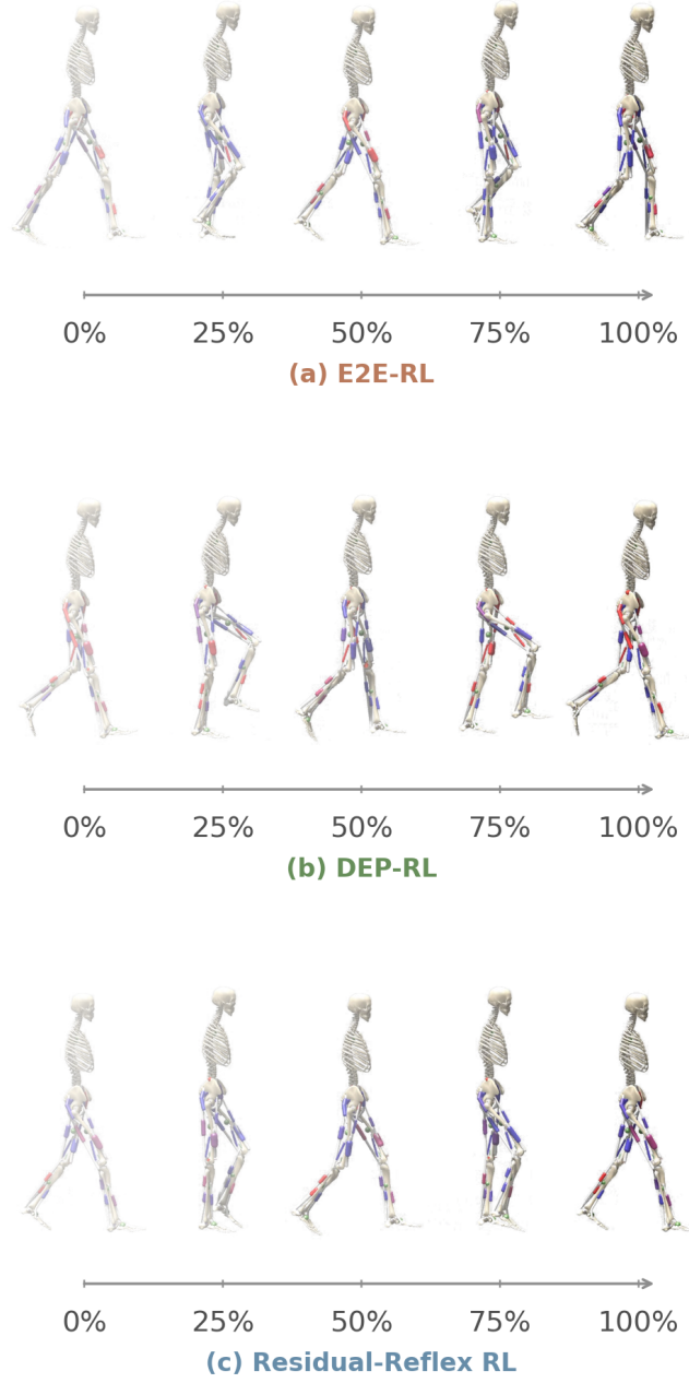
Figure 9: Qualitative gait snapshots over one detected gait cycle at 1.2 m/s for (a) E2E-RL, (b) DEP-RL, and (c) Residual-Reflex RL. Within each panel, frames were sampled at 0%, 25%, 50%, 75%, and 100% of the gait cycle detected from the corresponding STO trajectory and synchronized video.
