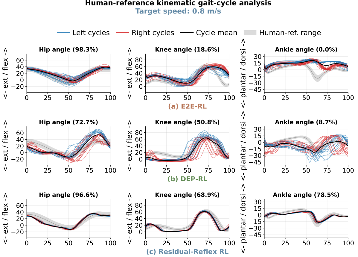
Figure 4: Human-reference kinematic gait-cycle visualization at target speed 0.8 m/s for E2E-RL, DEP-RL, and Residual-Reflex RL. Blue and red curves denote left and right gait cycles, respectively; the black curve is the cycle average and the gray band is the human-reference range. Horizontal axes show normalized gait cycle percentage.
