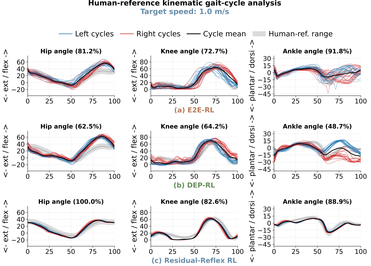
Figure 5: Human-reference kinematic gait-cycle visualization at target speed 1.0 m/s for E2E-RL, DEP-RL, and Residual-Reflex RL. Blue and red curves denote left and right gait cycles, respectively; the black curve is the cycle average and the gray band is the human-reference range. Horizontal axes show normalized gait cycle percentage.
