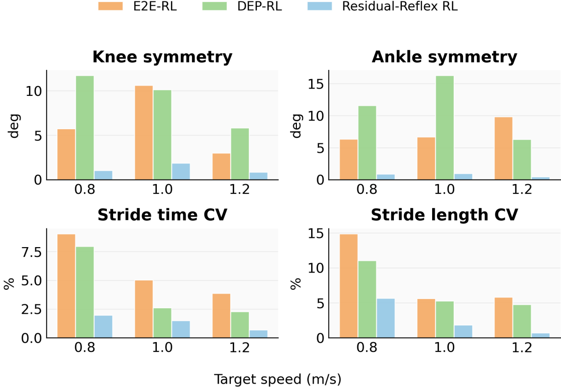
Figure 8: Left–right waveform differences and stride variability across target speeds. Lower values indicate more symmetric and more repeatable gait cycles.
