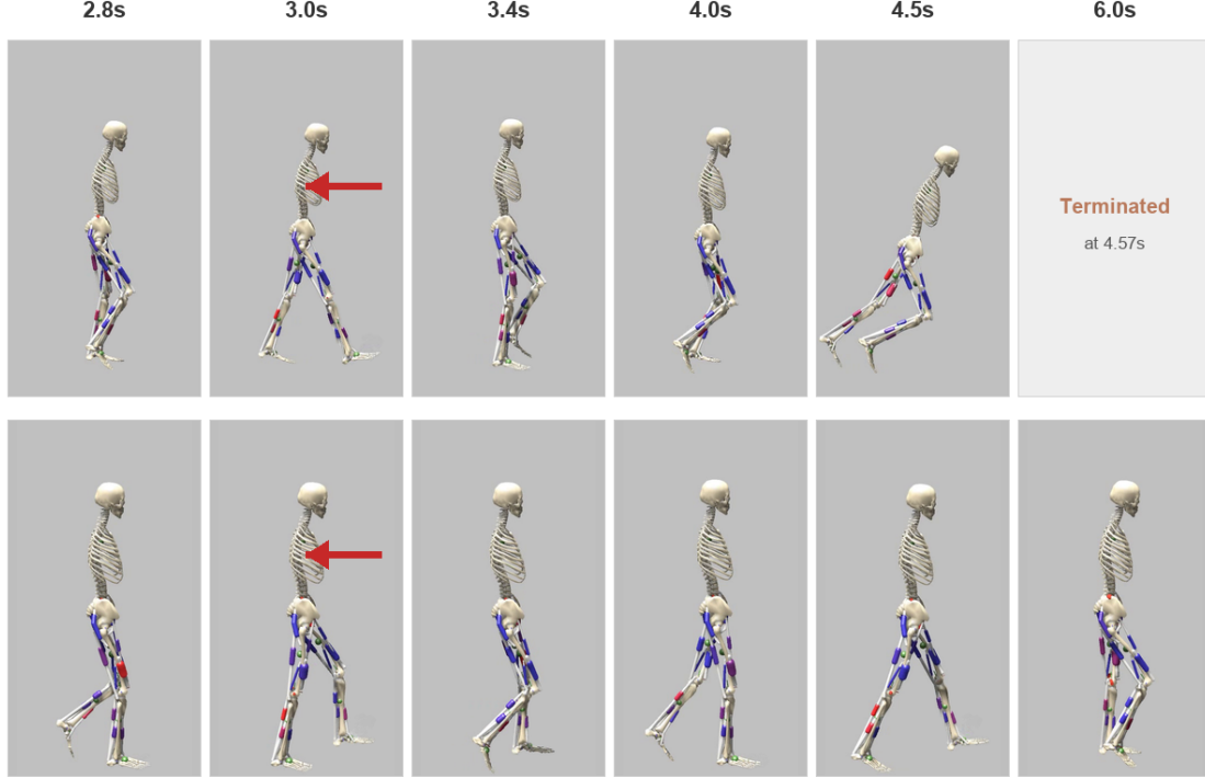
Figure 13: Time-aligned response to a 100 N backward torso push applied for 0.1 s at t = 3.0 s. Columns show synchronized frames from 2.8 s to 6.0 s. The CMA-ES-optimized reflex controller (top) progressively loses upright balance and terminates at 4.57 s. Residual-Reflex RL (bottom) modifies the following steps and continues walking for the full 25 s rollout under the same perturbation. Red arrows indicate the applied force.
