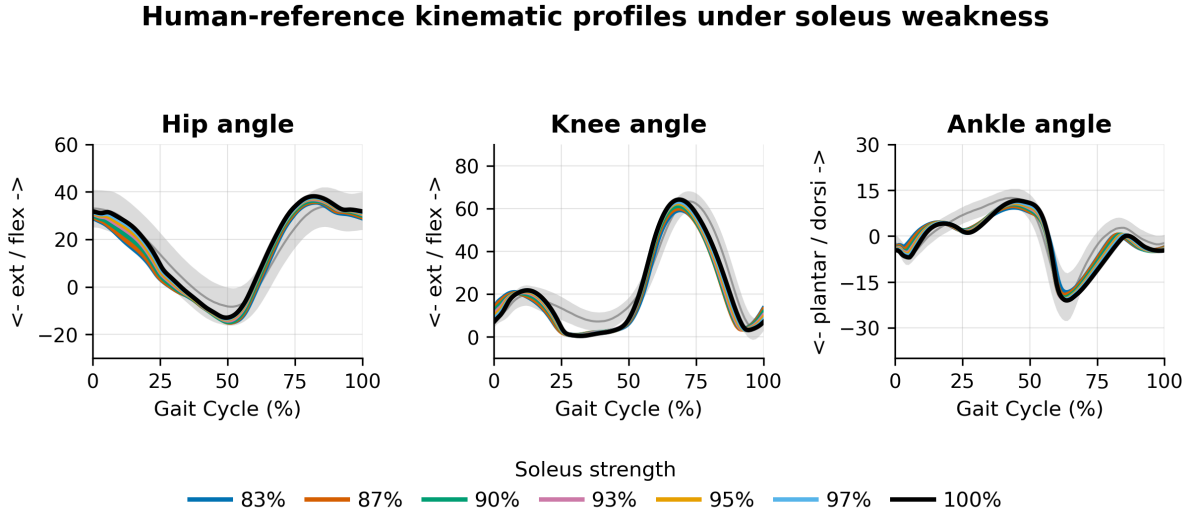
Figure 12: Human-reference kinematic profiles under soleus weakness. Colored curves show the mean normalized gait-cycle profiles generated by the same trained Residual-Reflex RL policy under different soleus strength levels; the gray bands denote the human-reference ranges.
