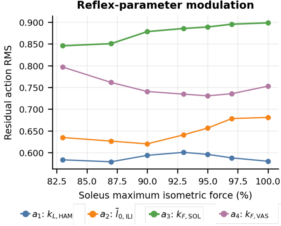
Figure 11: Residual-action modulation under plantarflexor weakness. RMS values show that the trained policy continues to adjust all four selected reflex channels. Channel a_3 modulates soleus force feedback for ankle support/propulsion, whereas a_4 modulates vasti force feedback for knee extension and stance support.
