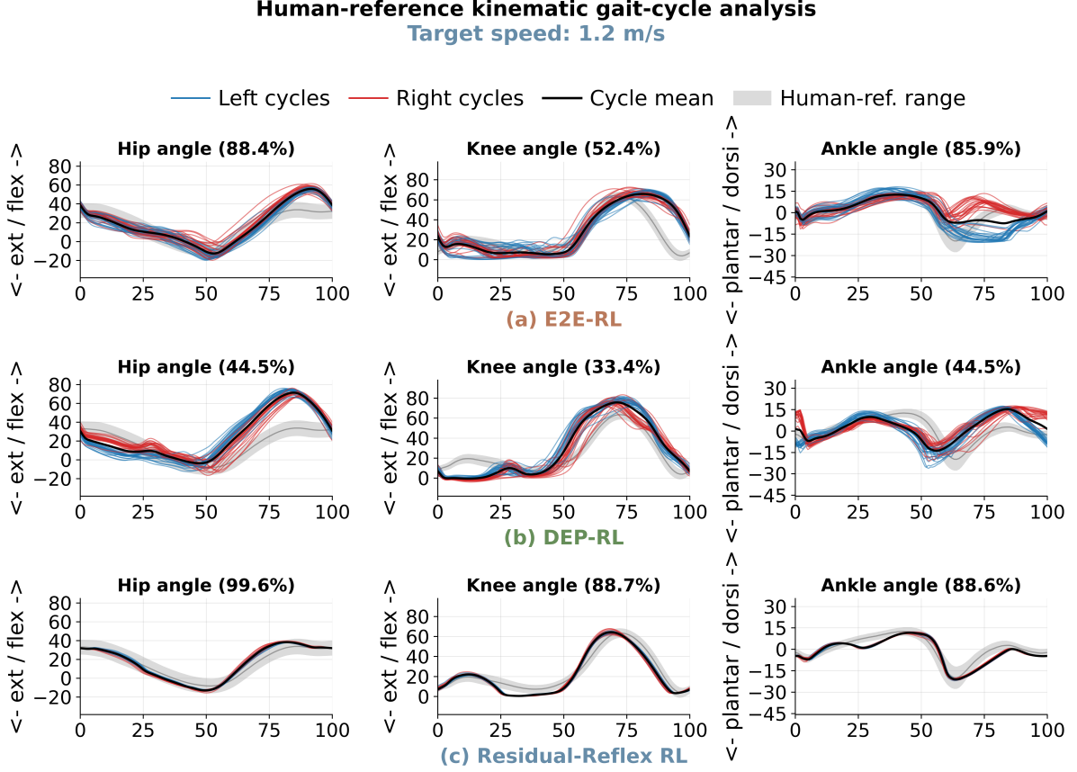
Figure 6: Human-reference kinematic gait-cycle visualization at target speed 1.2 m/s for E2E-RL, DEP-RL, and Residual-Reflex RL. Blue and red curves denote left and right gait cycles, respectively; the black curve is the cycle average and the gray band is the human-reference range. Horizontal axes show normalized gait cycle percentage.
