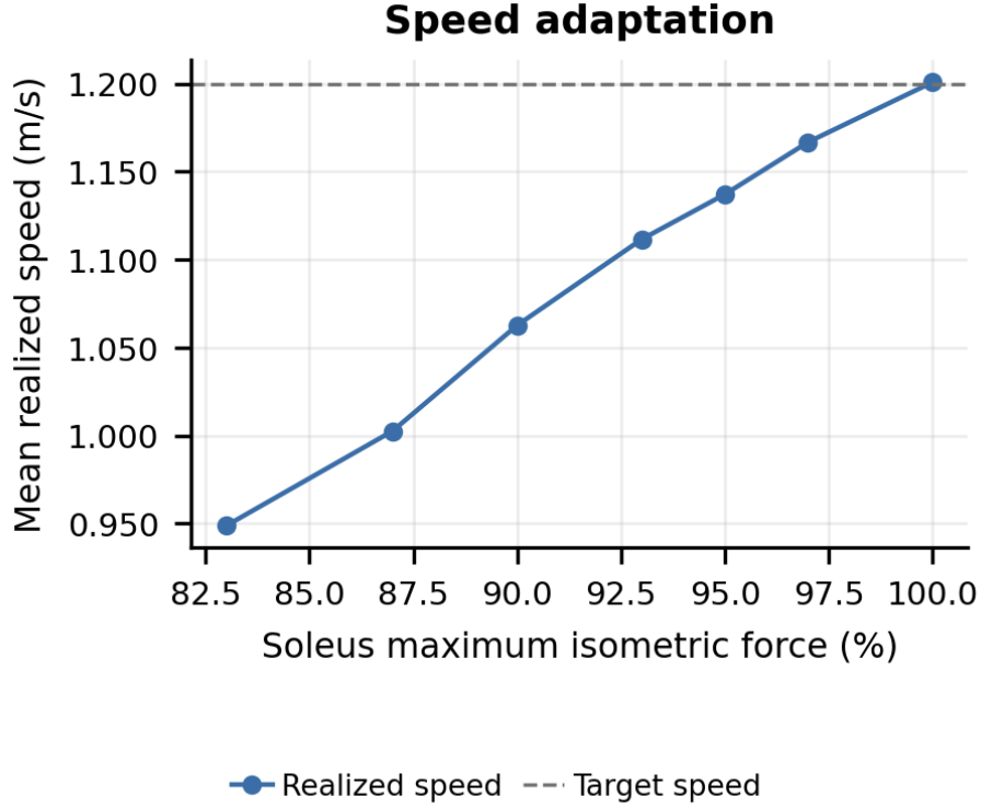
Figure 10: Speed adaptation under plantarflexor weakness. The same trained Residual-Reflex RL policy remains stable across weakened soleus models but adopts a slower realized speed as force capacity is reduced.
