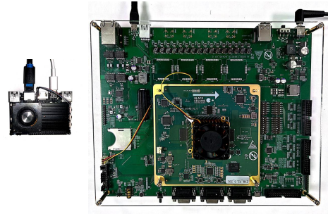
Fig. 6. Picture of Khadas VIM3 Pro board (left) and BST A1000 evaluation board (right).
