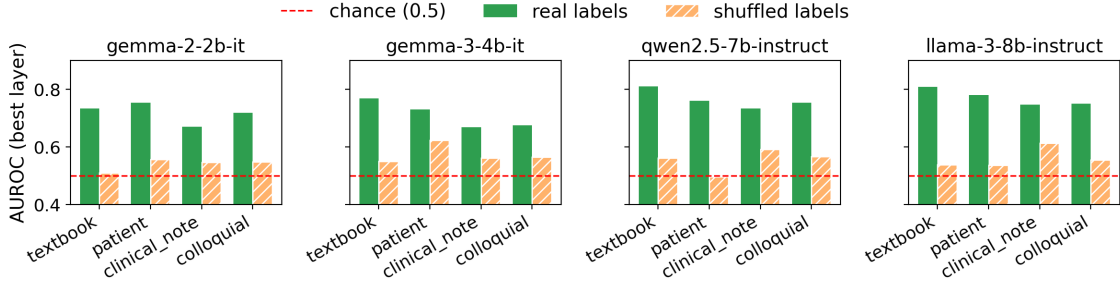
Figure 10: Permutation sanity check. Green: real-label probe. Orange hatched: label-shuffled. Red dashed: chance (0.5). Mean permuted AUROC over all layers is 0.488.
