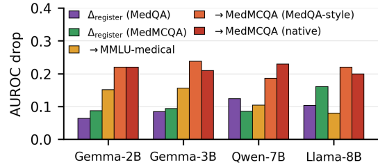
Figure 3: The three shifts side by side, per LLM. Purple: within-MedQA register \Delta_{\text{register}} ( n=500 ). Green: within-MedMCQA register \Delta_{\text{register}} ( n=100 ). Red: MedQA-to-MedMCQA \Delta_{\text{dataset}} ; yellow and orange: the same probe on MMLU-medical and on MedMCQA re-formatted into MedQA style.
