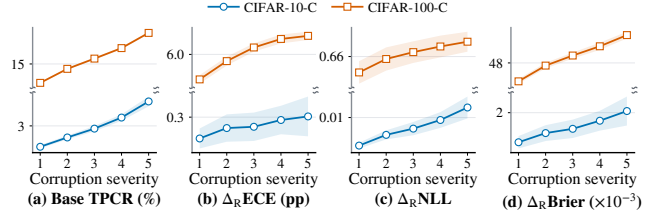
Figure 3: Base TPCR and paired metric reductions from CORD across corruption severity on CIFAR-10-C and CIFAR-100-C. For M \in \{\text{ECE}, \text{NLL}, \text{Brier}\} , \Delta_R M = M(\text{Base}) - M(\text{Base} + \text{CORD}) , with \Delta_R M > 0 indicating improvement. Curves average over classifiers, calibrators, and 15 corruptions; shading shows pointwise 95% CIs.
