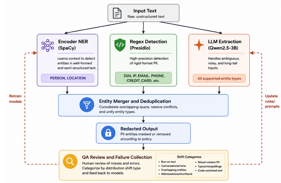
Fig. 2. Proposed hybrid PII detection pipeline. Three architectural families run in parallel, their outputs are merged, and a QA feedback loop iteratively improves each component based on categorized production failures.
